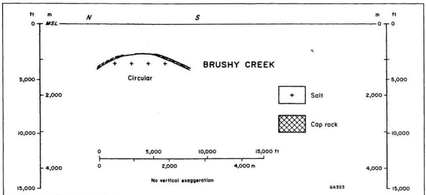
Figure 34. Cross section through Brushy Creek salt stock, which is axially symmetric.
