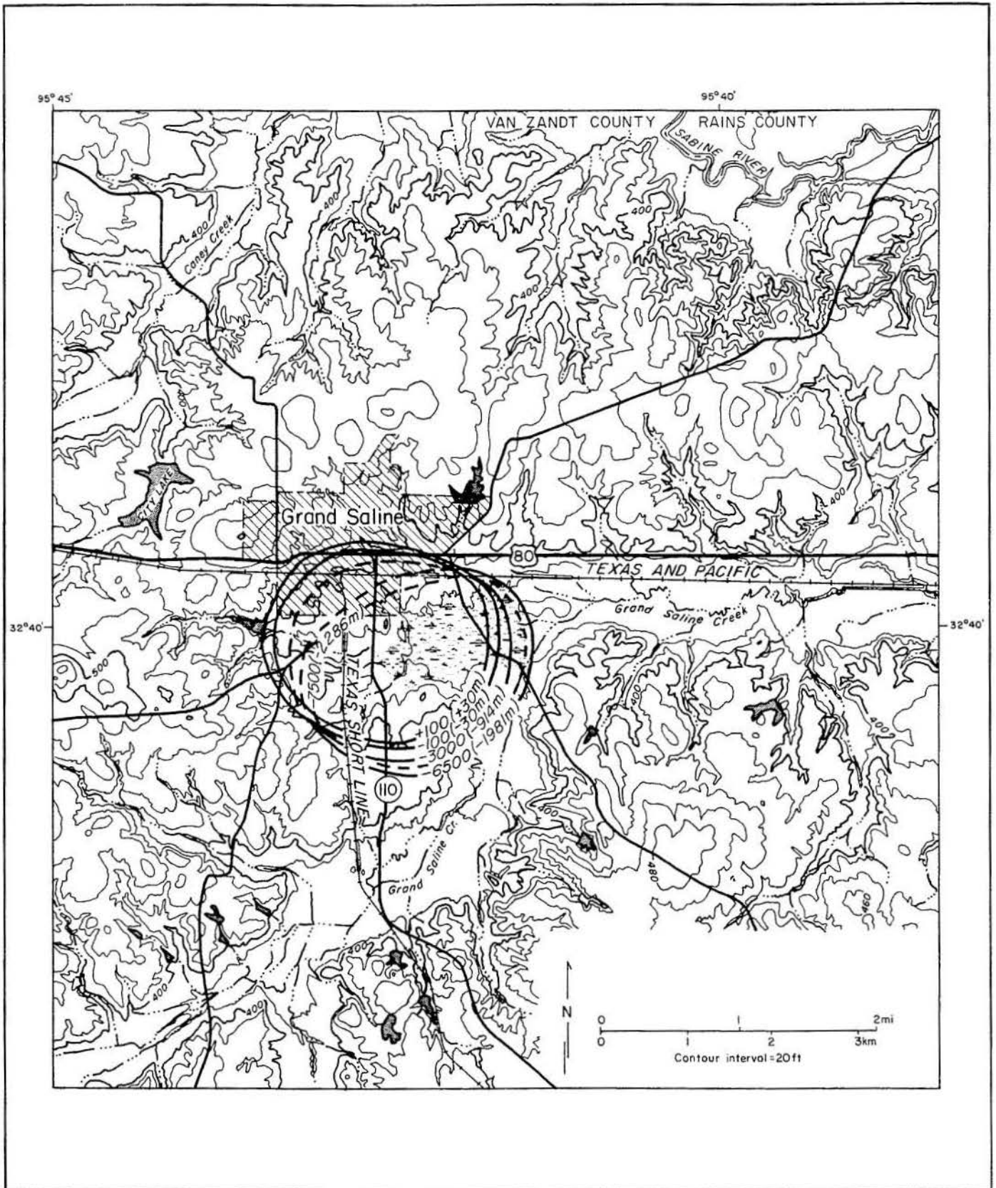
Figure 48. Map showing shape, location, topography, and drainage system of Grand Saline Dome (salt structure contours from Giles, 1980).
