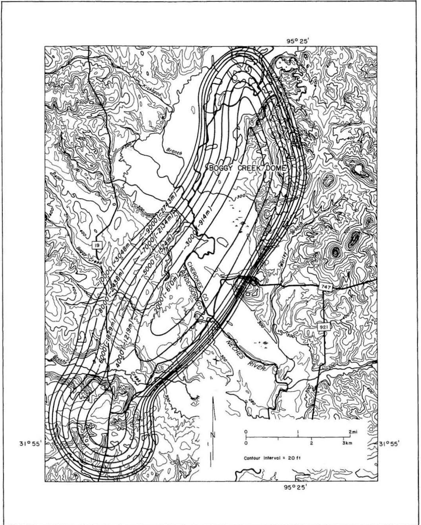
Figure 24. Map showing shape, location, topography, and drainage system of Bogy Creek Dome (salt structure contours from Giles, 1981).
