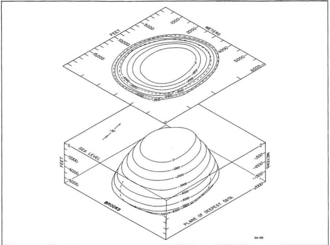
Figure 29. Isometric block diagram of Brooks salt stock.
