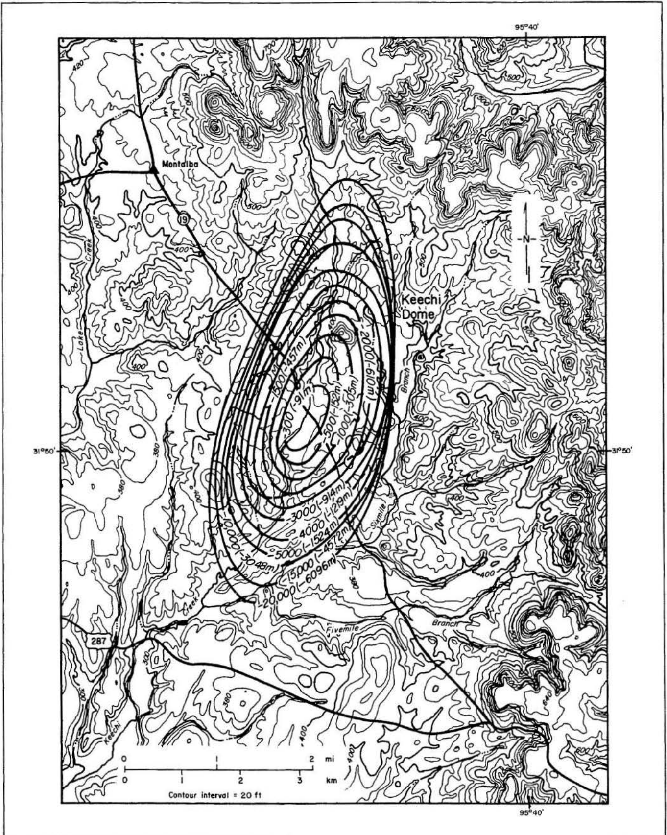
Figure 57. Map showing shape, location, topography, and drainage system of Keechi Dome (salt structure contours modified from Exploration Techniques, 1979).
