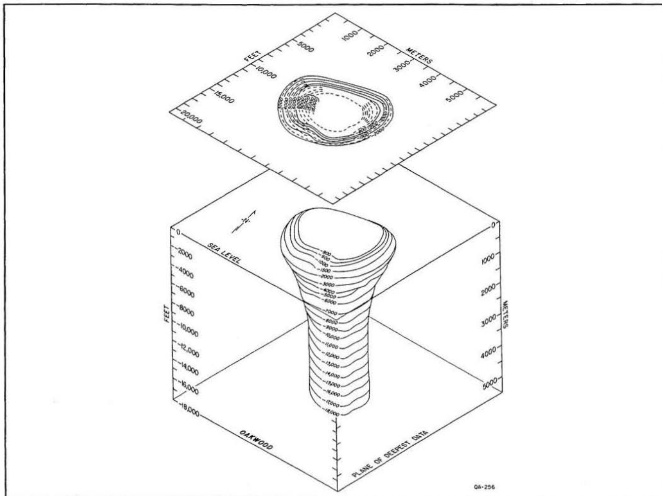
Figure 66. Isometric block diagram of Oakwood salt stock.
