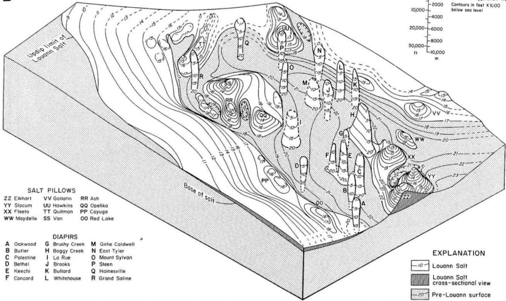
Figure 4. Isometric block diagrams of the East Texas Basin showing three-dimensional configuration of structure contours on top of the Louann Salt or on top of the pre-Louann surface where salt is thin or absent. Where indicated as "absent," the Louann Salt is too thin to be seismically resolved into a discrete unit or is too thin to supply further salt to diapirs; its actual thickness here may be as much as a few hundred feet. (A) Northwest view. (B) Northeast view. Constructed by isometric projection and incremental translation of contours, following Lobeck (1924, p. 138-142). (A) From Jackson and Seni (1983). (B) From Seni and Jackson (1984).
