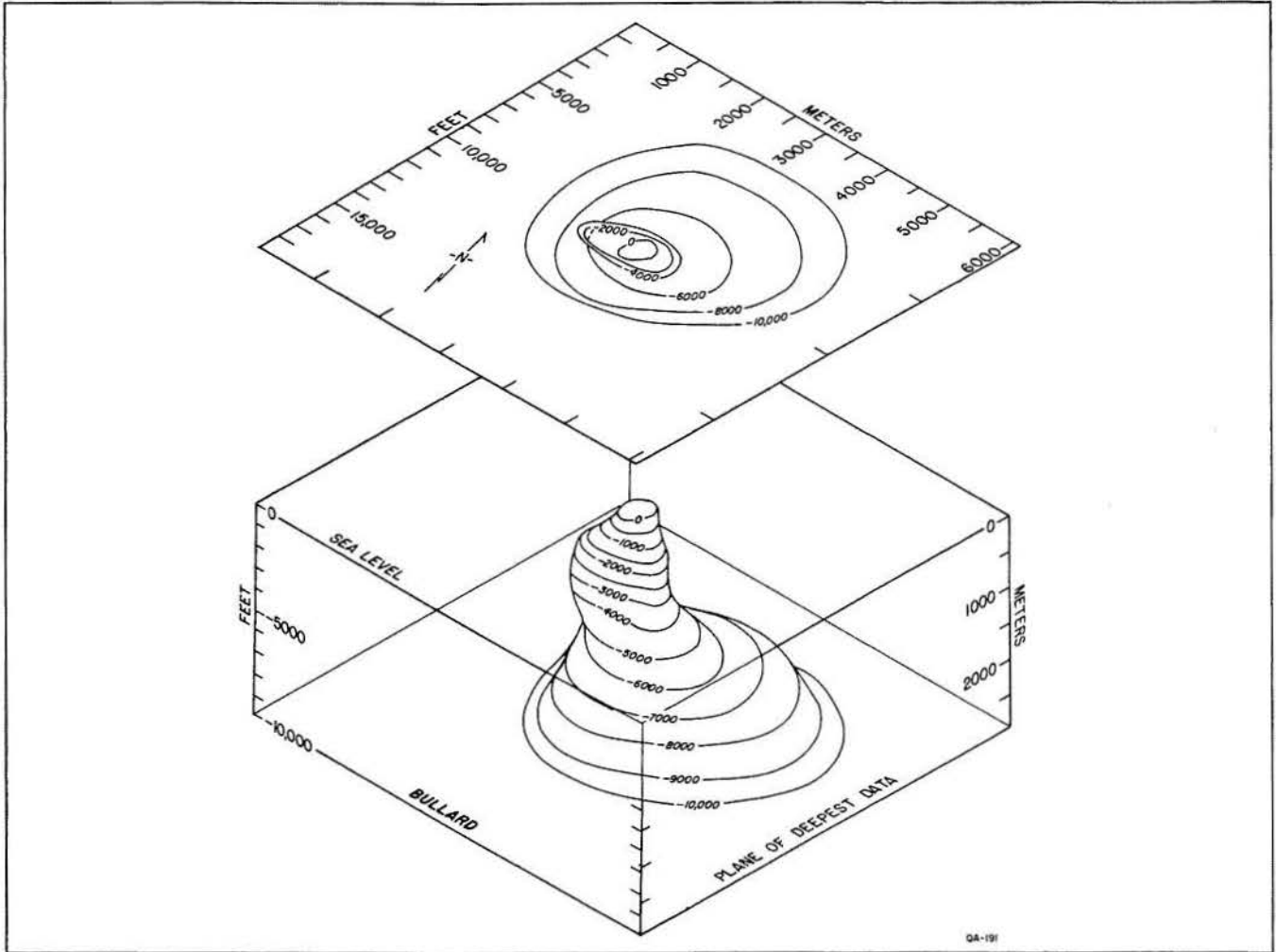
Figure 37. Isometric block diagram of Bullard salt stock.
