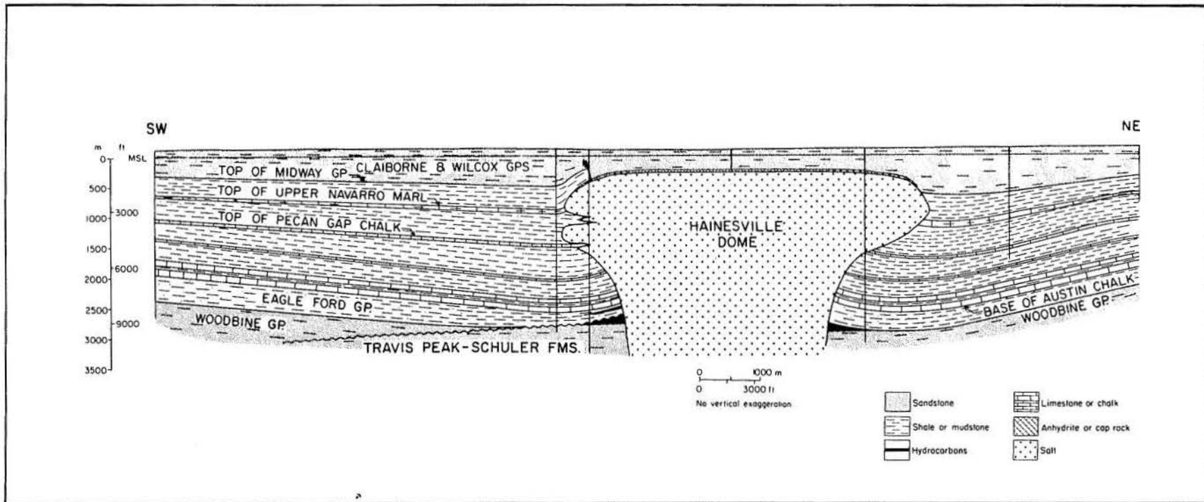
Figure 55. Structural cross section through Hainesville Dome, based on drilling data (Giles and Wood, 1981).
