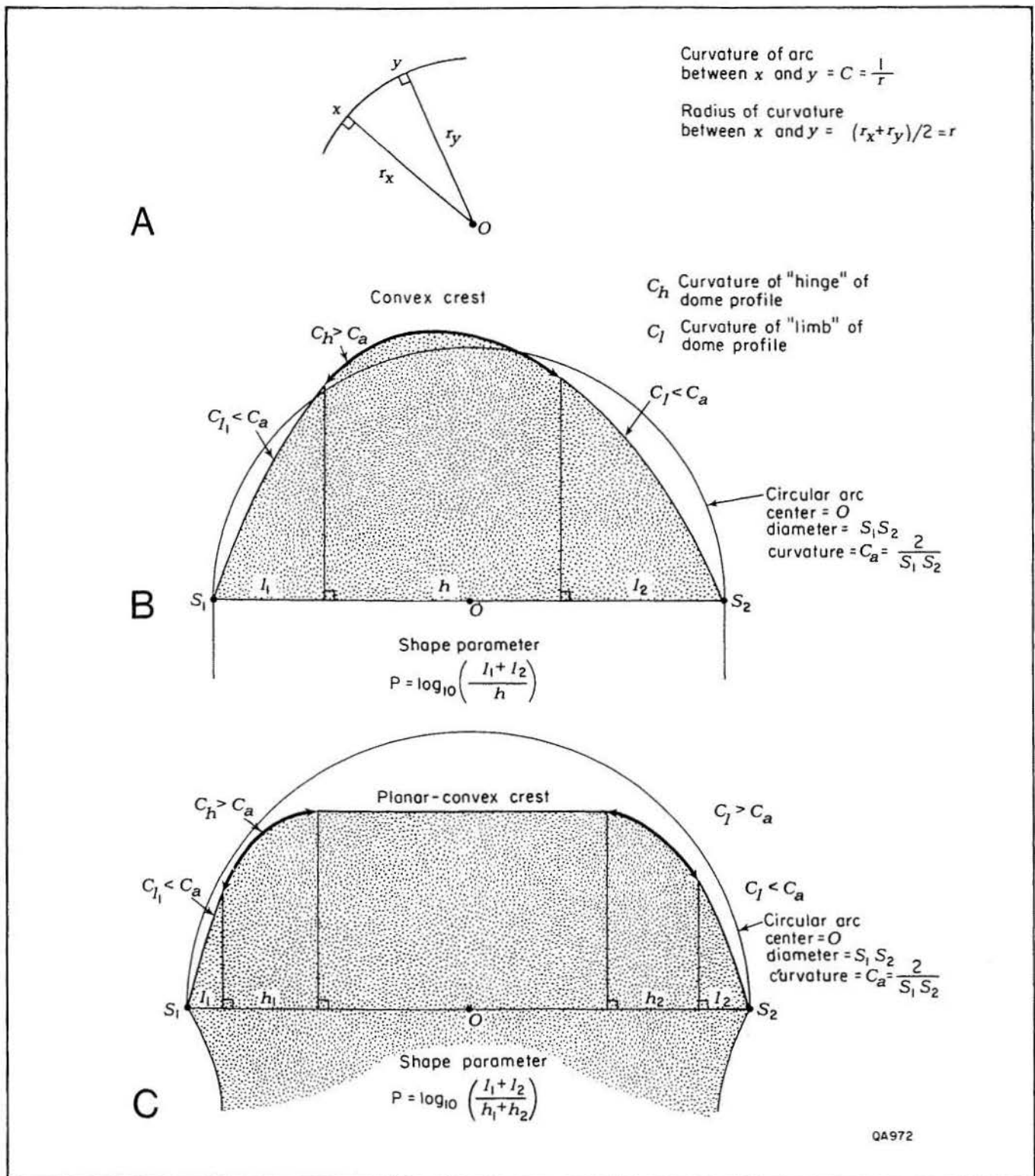
Figure 11. Derivation of a shape parameter to differentiate between diapir crests with straight or slightly curved sides and crests with strongly curved sides. (A) Calculation of curvature and radius of curvature between two points, x and y , on an arc (after Ramsay, 1967, fig. 7-7). (B) Calculation of the shape parameter in a cross section of a dome (stippled) having a nonplanar crest. The arc shown in heavy line has curvature greater than that of a circular arc and corresponds geometrically (not mechanically) to the hinge of a folded surface. (C) Calculation of the shape parameter in a cross section of a dome (stippled) having a crest with sloping sides and a planar, horizontal upper surface. The horizontal part is not involved in the calculation, and the shape parameter is independent of the percentage planar crest. Designating the shape parameter as a log allows values to vary symmetrically each side of zero.
