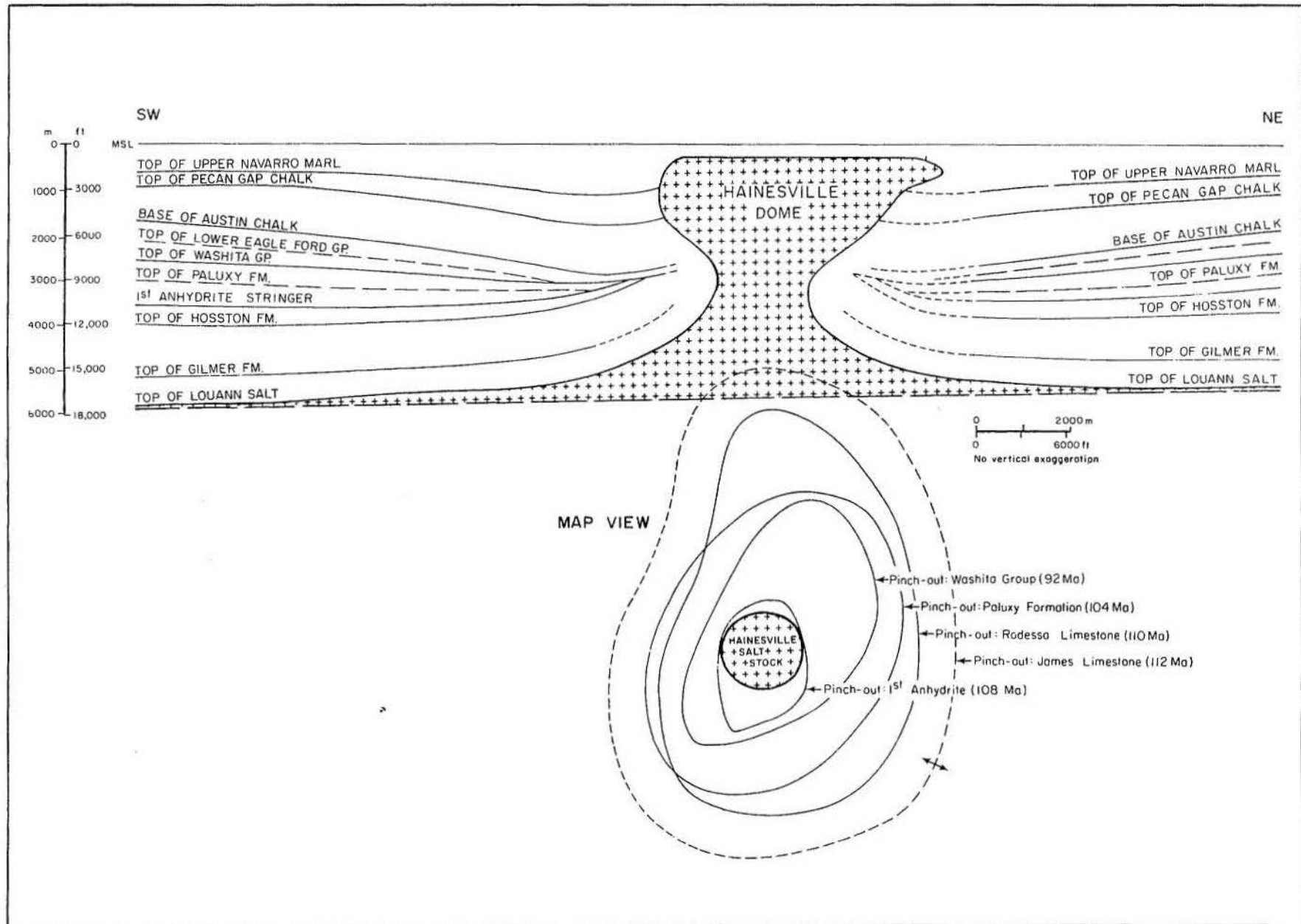
Figure 56. Structural cross section through Hainesville Dome, based on seismic data. (After Loocke, 1978.)
