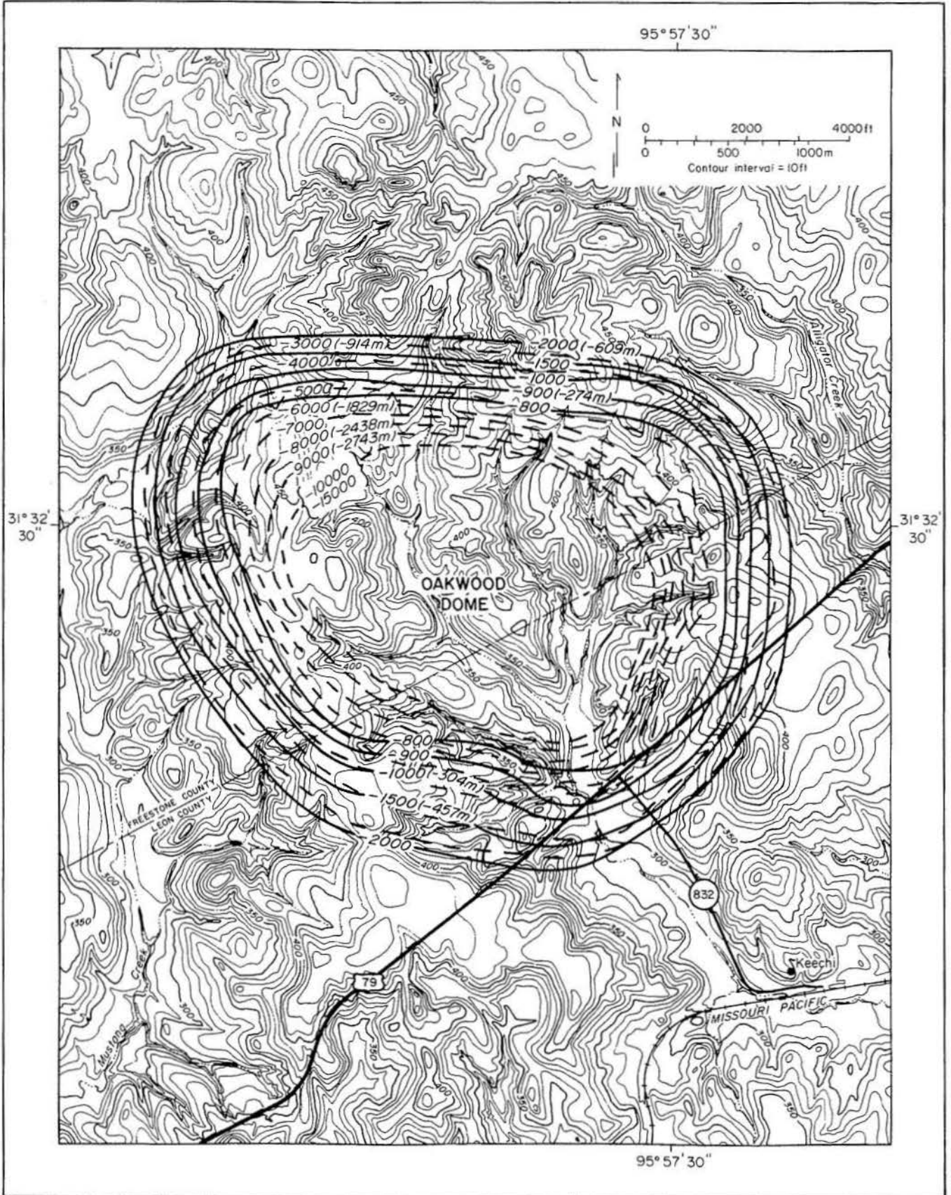
Figure 65. Map showing shape, location, topography, and drainage system of Oakwood Dome (salt structure contours modified from Exploration Techniques, 1979).
