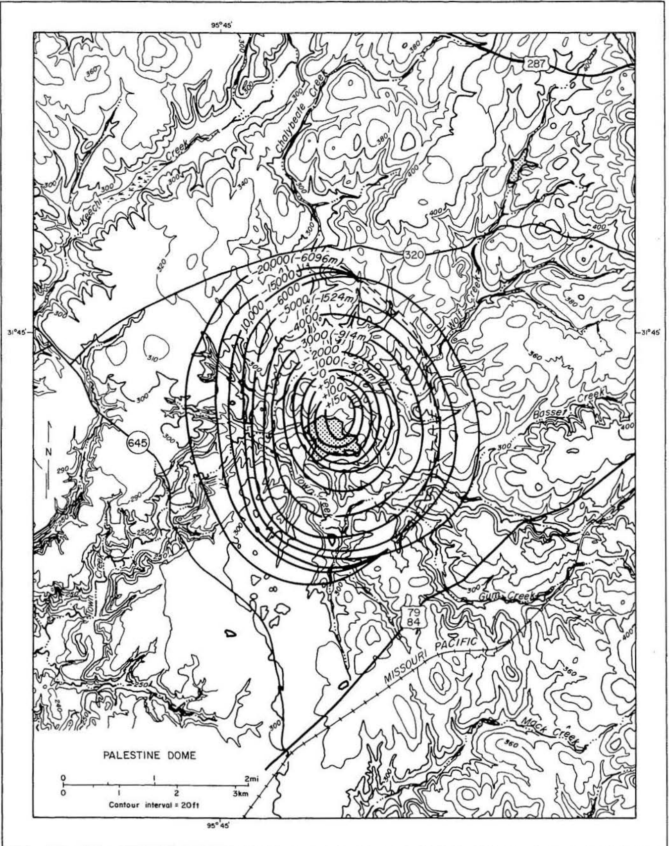
Figure 69. Map showing shape, location, topography, and drainage system of Palestine Dome (salt structure contours from Giles, 1980).
