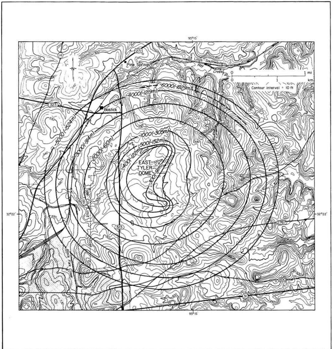
Figure 44. Map showing shape, location, topography, and drainage system of East Tyler Dome (salt structure contours from Giles, 1980).
