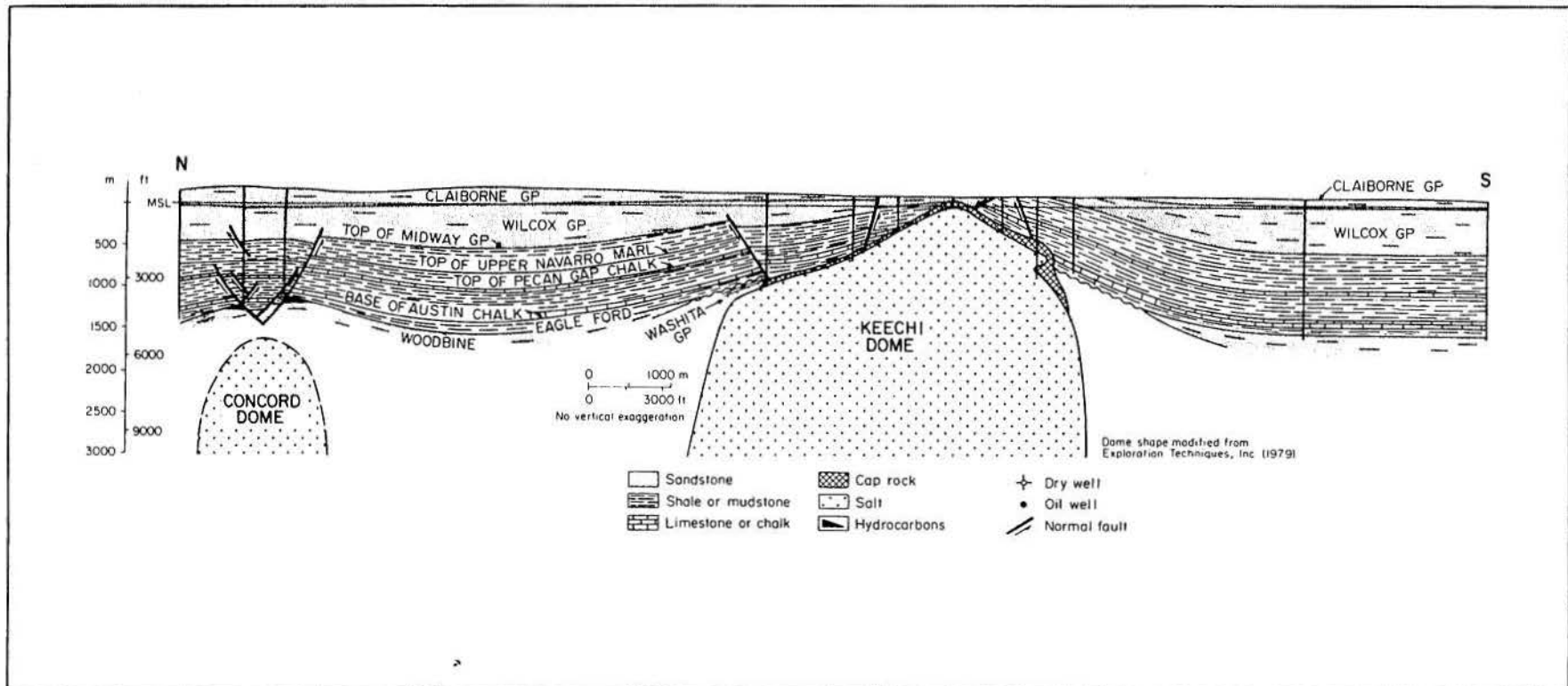
Figure 60. Structural cross section through Keechi Dome and Concord Dome, a deep-diapir area (Giles and Wood, 1981).
