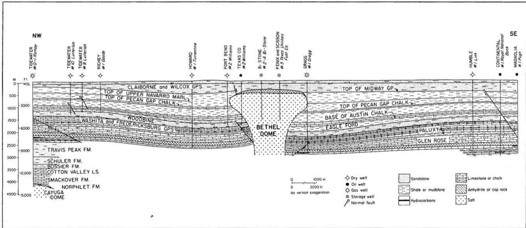
Figure 23. Structural cross section through Bethel Dome (Wood and Giles, 1982).
