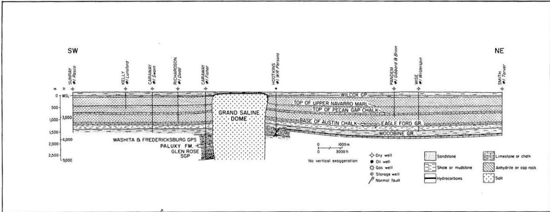
Figure 51. Structural cross section through Grand Saline Dome (Giles and Wood, 1981).
