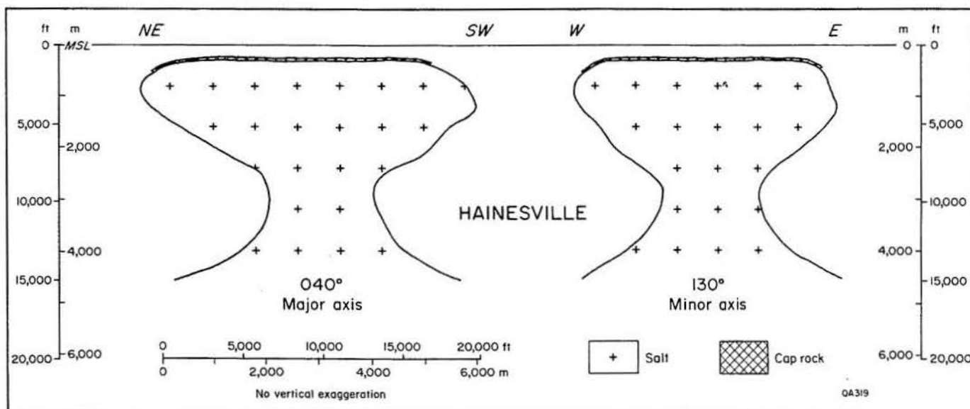
Figure 54. Orthogonal cross sections through major and minor axes of Hainesville salt stock.
