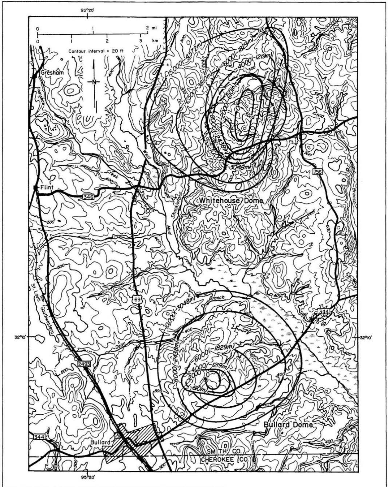
Figure 36. Map showing shapes, locations, topography, and drainage systems of Bullard and Whitehouse Domes (salt structure contours from Netherland, Sewell and Associates, 1976).
