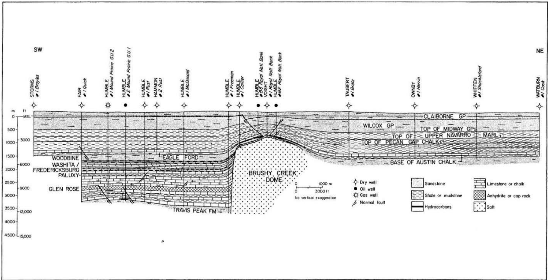
Figure 35. Structural cross section through Brushy Creek Dome (Wood and Giles, 1982).
