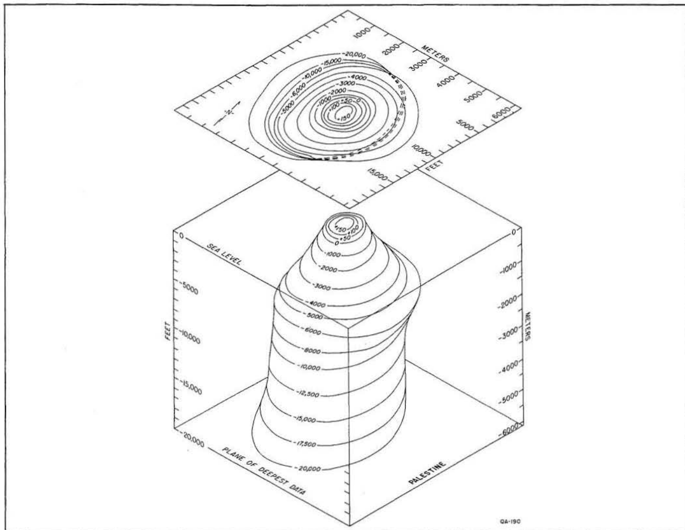
Figure 70. Isometric block diagram of Palestine salt stock.
