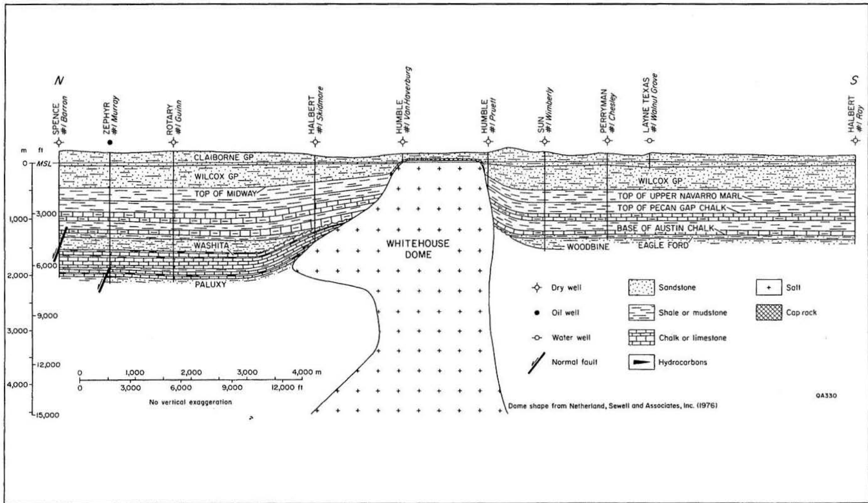
Figure 79. Structural cross section through Whitehouse Dome (Giles, 1980).
