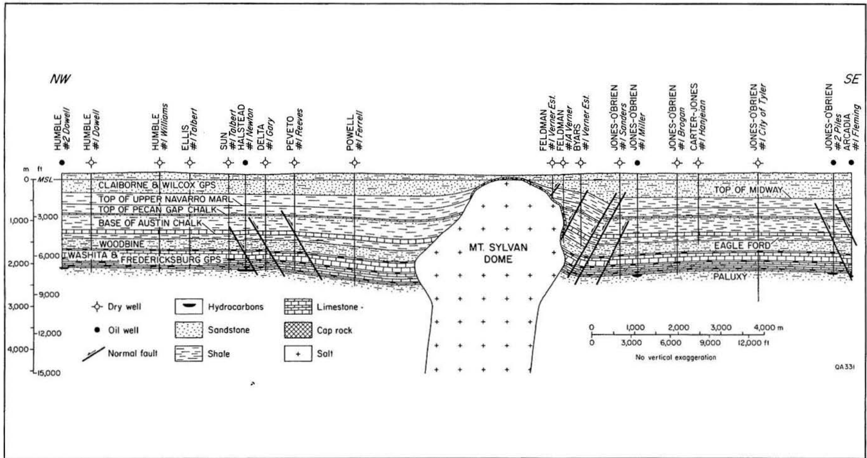
Figure 64. Structural cross section through Mount Sylvan Dome (Giles, 1980).
