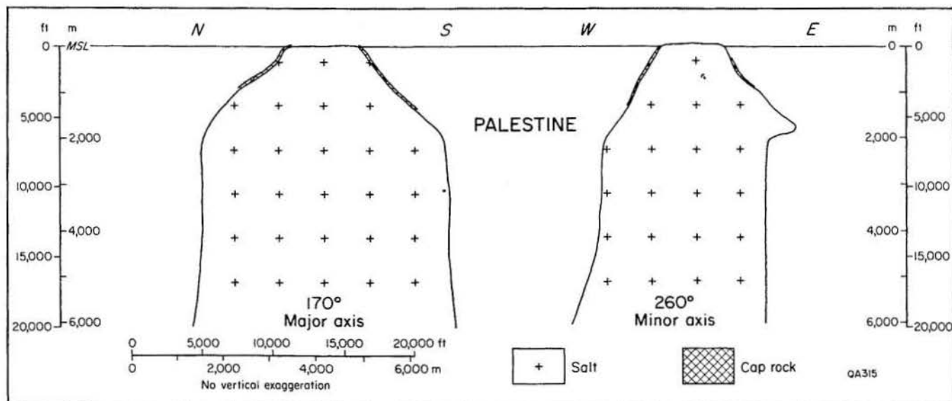
Figure 71. Orthogonal cross sections through major and minor axes of Palestine salt stock.
