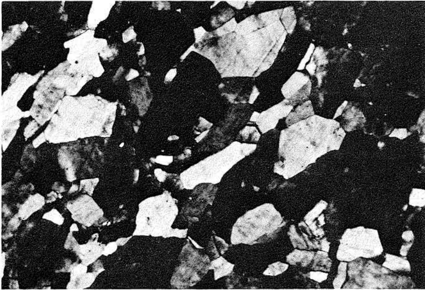
FIGURE 45. Fine-grained gypsum from Rayburn's Dome cap rock; depth is 77 ft (23.5 m). Photo width is 2.0 mm; crossed nicols.
