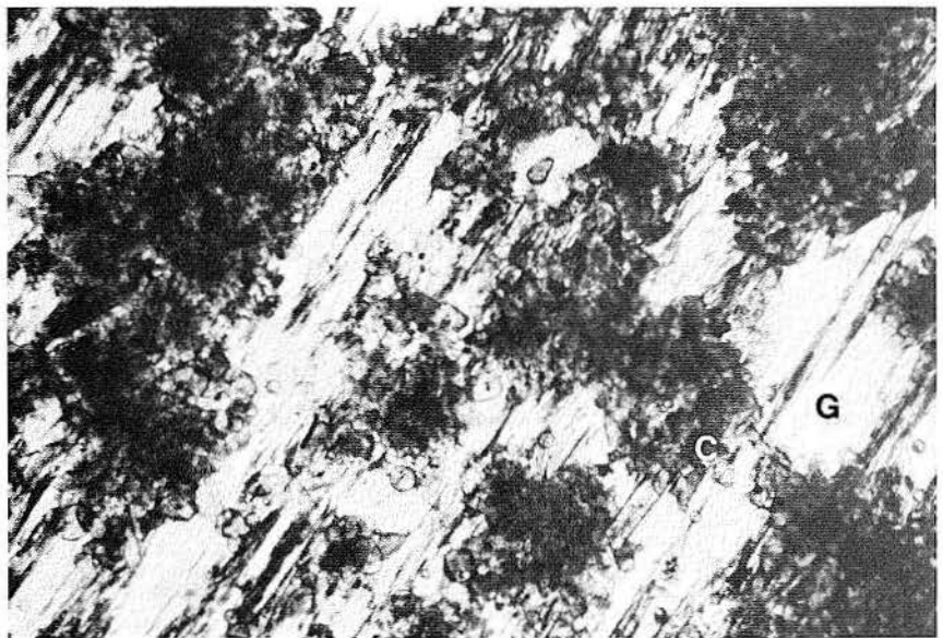
FIGURE 30. Fibrous gypsum (G) and fine-grained, calcite (C) in anhydrite-calcite transition zone, Oakwood cap rock; depth is 907 ft (276.5 m). Photo width is 2.6 mm; plane light.
