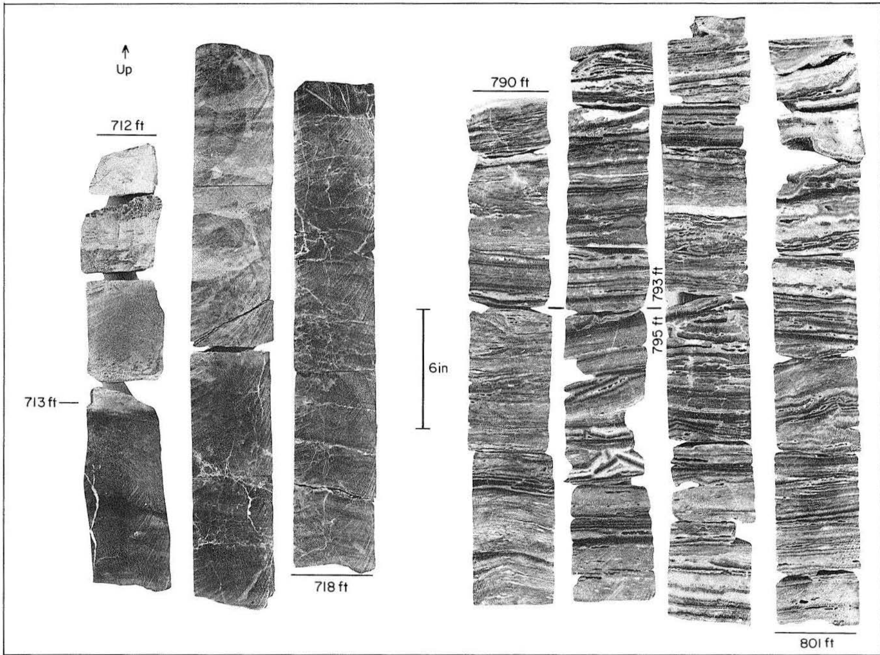
FIGURE 20. Core photographs of Oakwood cap rock. Depths are in feet.
