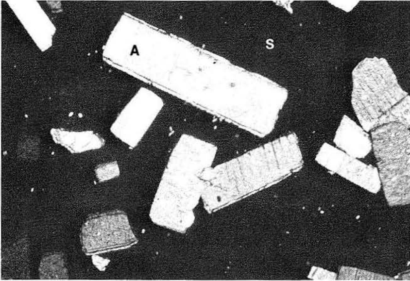
FIGURE 5. Anhydrite crystals (A) within Gyp Hill salt stock (S); depth is 915 ft (278.9 m). Photo width is 2.6 mm; crossed nicols.
