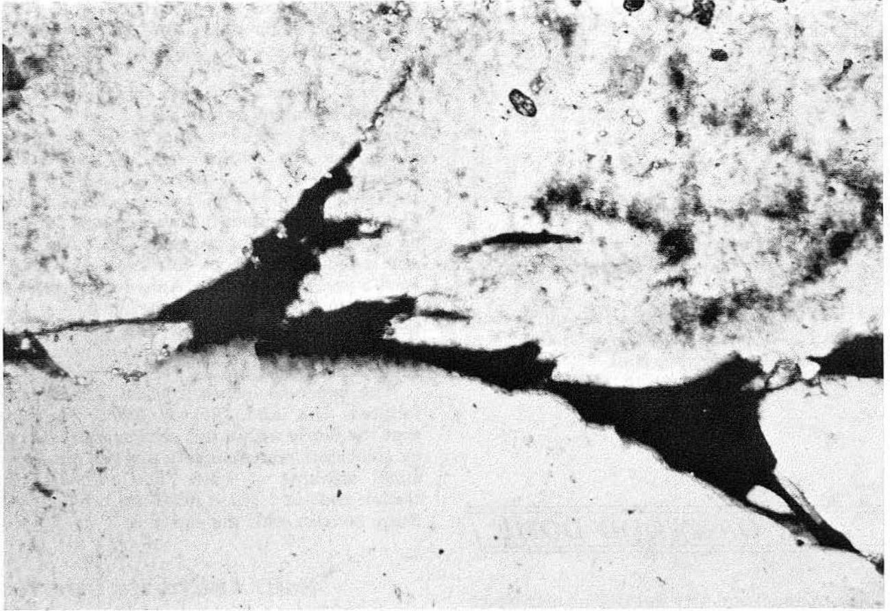
FIGURE 16. Shear fractures in gypsum from Gyp Hill cap rock; depth is 308 ft (93.9 m). Photo width is 2.6 mm; crossed nicols.
