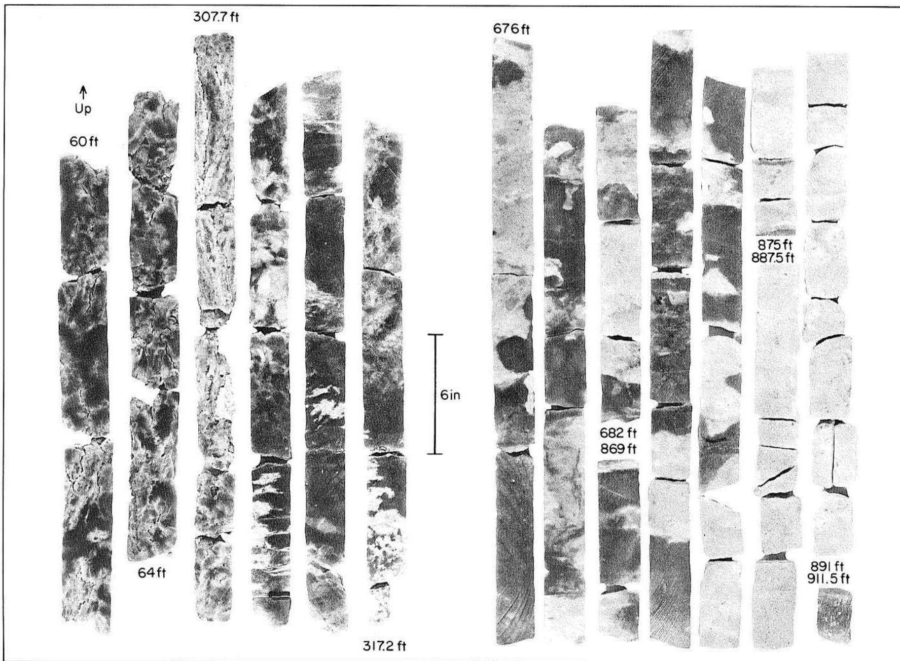
FIGURE 7. Core photographs of Gyp Hill cap rock. Depths are in feet below land surface. See figure 8 for description.
