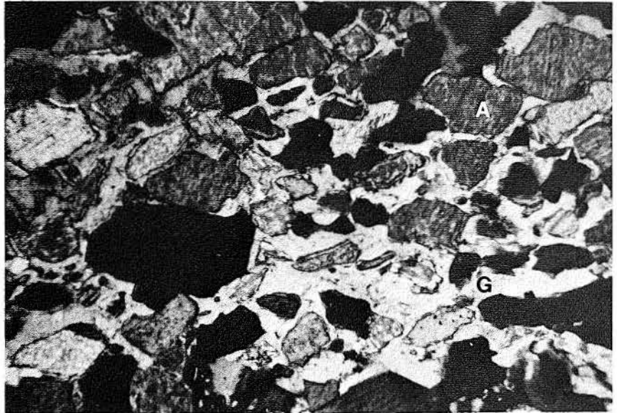
FIGURE 29. Poikilotopic gypsum cement (G) and anhydrite (A) in anhydrite-calcite transition zone, Oakwood cap rock; depth is 906 ft (276.1 m). Photo width is 2.6 mm; crossed nicols.
