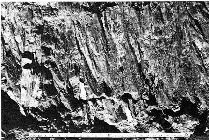
FIGURE 17. Strained gypsum, quarry wall, Gyp Hill salt dome.
