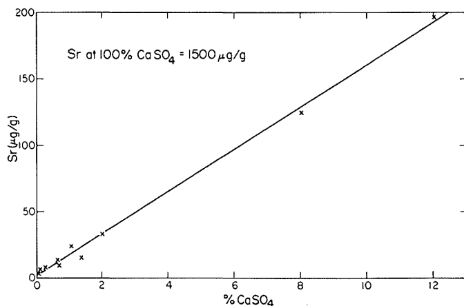
FIGURE 33. Strontium versus percent \text{CaSO}_4 in salt, Oakwood salt dome. If extrapolated to 100 percent \text{CaSO}_4 , the Sr content would be 1,500 \mu\text{g/g} .
