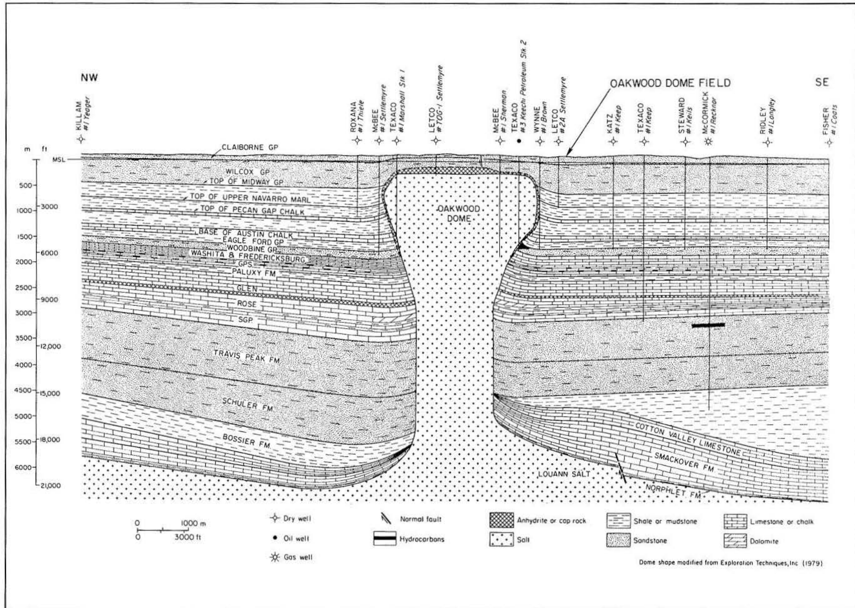
FIGURE 21. Geologic cross section of Oakwood salt dome (from Giles and Wood, 1983).
