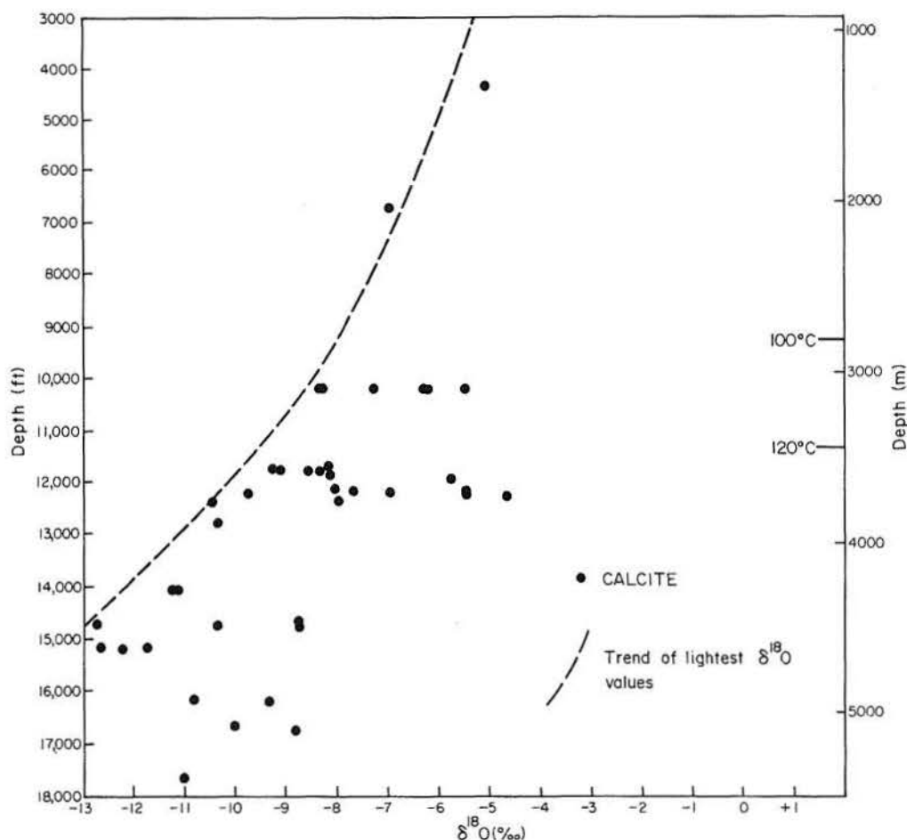
FIGURE 39. The \delta^{18}\text{O} (PDB) trend of calcite versus depth and temperature, Frio Formation, Texas Gulf Coast Milliken and others, 1981. Note the depletion of \delta^{18}\text{O} with depth.
