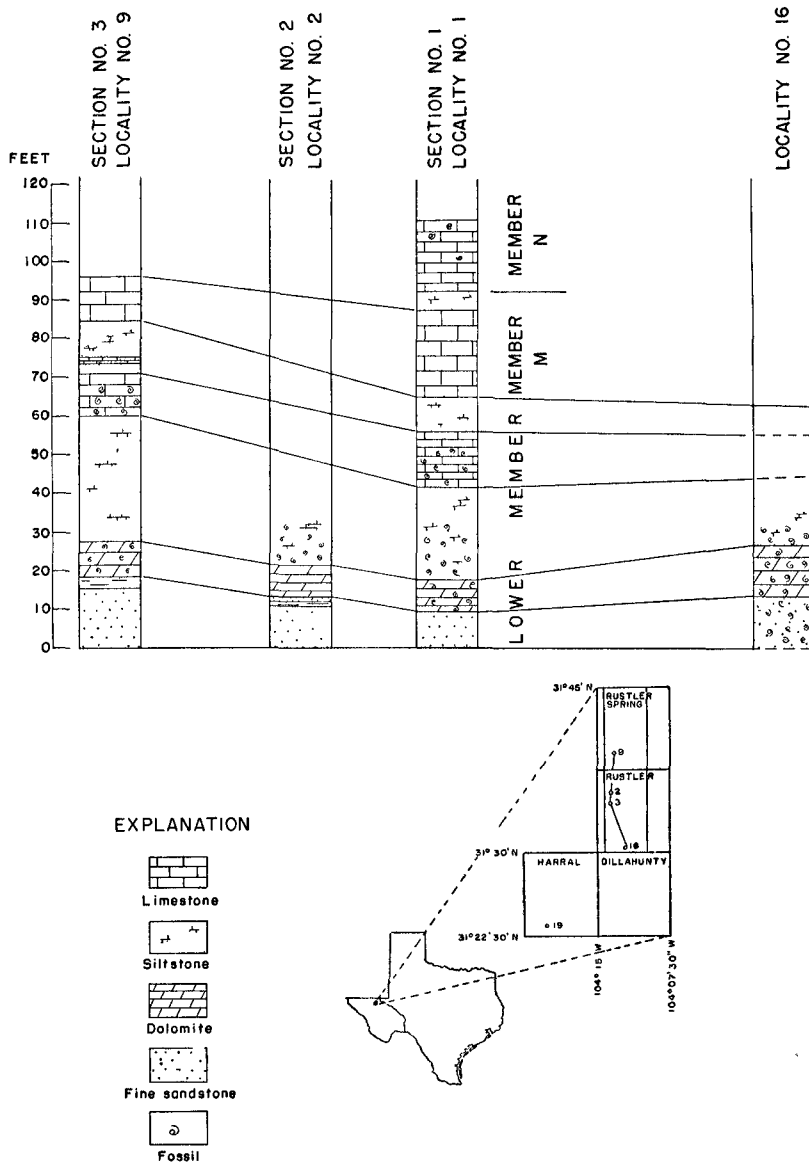
FIG. 2—Correlation of Rustler section, Culberson County, Texas. Datum: Base of sandstone lentil of lower member of Rustler formation. Horizontal distance not to scale.
