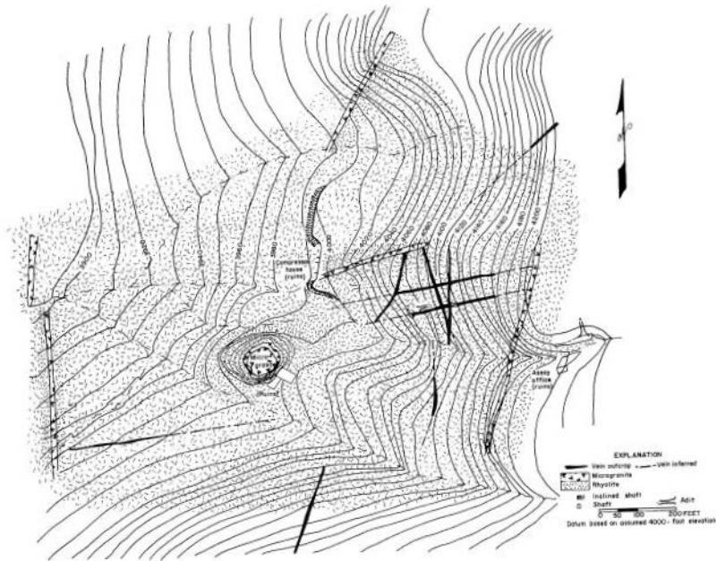
Figure 9. Area of San Antonio "mine," alidade survey.
