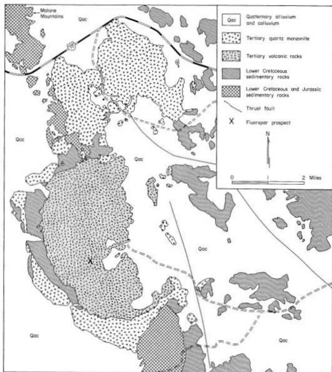
Figure 19. Geologic map, northern Quitman Mountains.
