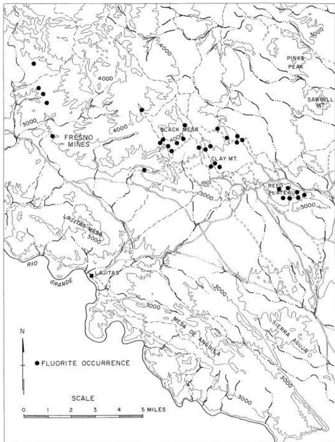
Figure 5. Fluorite occurrences in the Terlingua quicksilver district, Trans-Pecos Texas.
