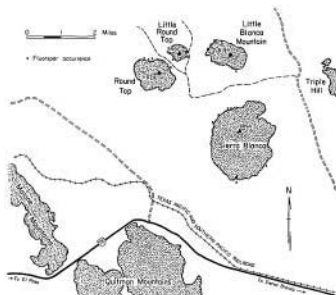
Figure 17. Sierra Blanca peaks district, Hudspeth County.
