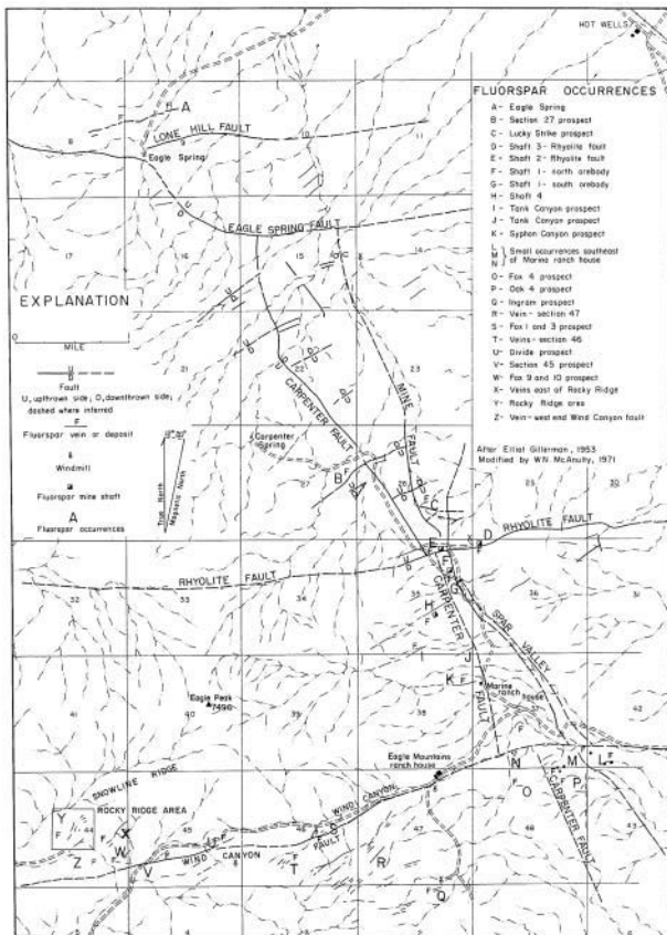
Figure 13. Eagle Mountains fluorspar district.
