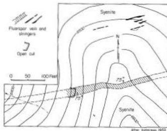
Figure 15. Fox 1 and 3 prospects.
