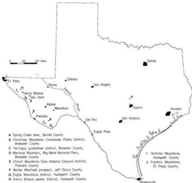
Figure 2. Fluorspar in Texas.
