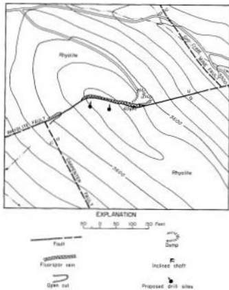
Figure 14. Rhyolite fault zone (after Gillerman, 1953).
