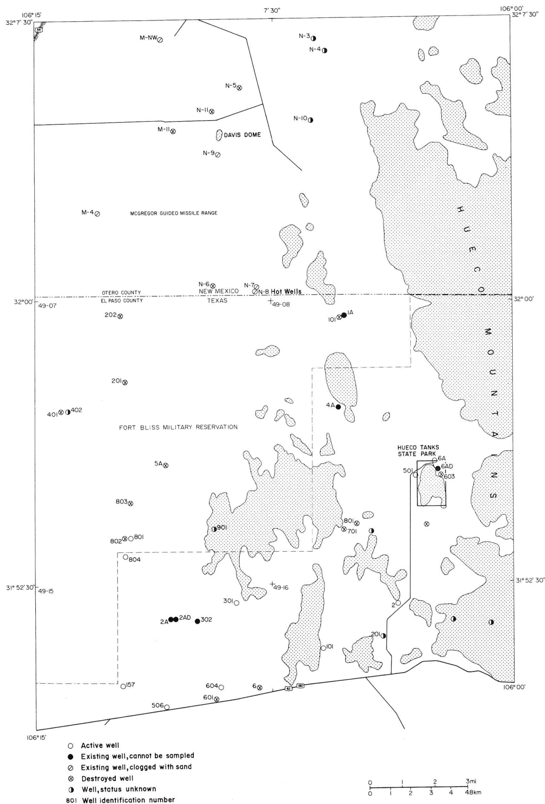
Figure 2. Wells in Hueco Tanks geothermal area. Well status symbols are also used on figures 3, 4, 5, 6, and 8. Wells in Texas are prefixed by a four-digit code that identifies the quadrangle in which the well occurs. This number is shown in the northwest corner of each quadrangle (for example, 49-07 at approximately lat 32^{\circ} N. and long 106^{\circ} 15' W.).
