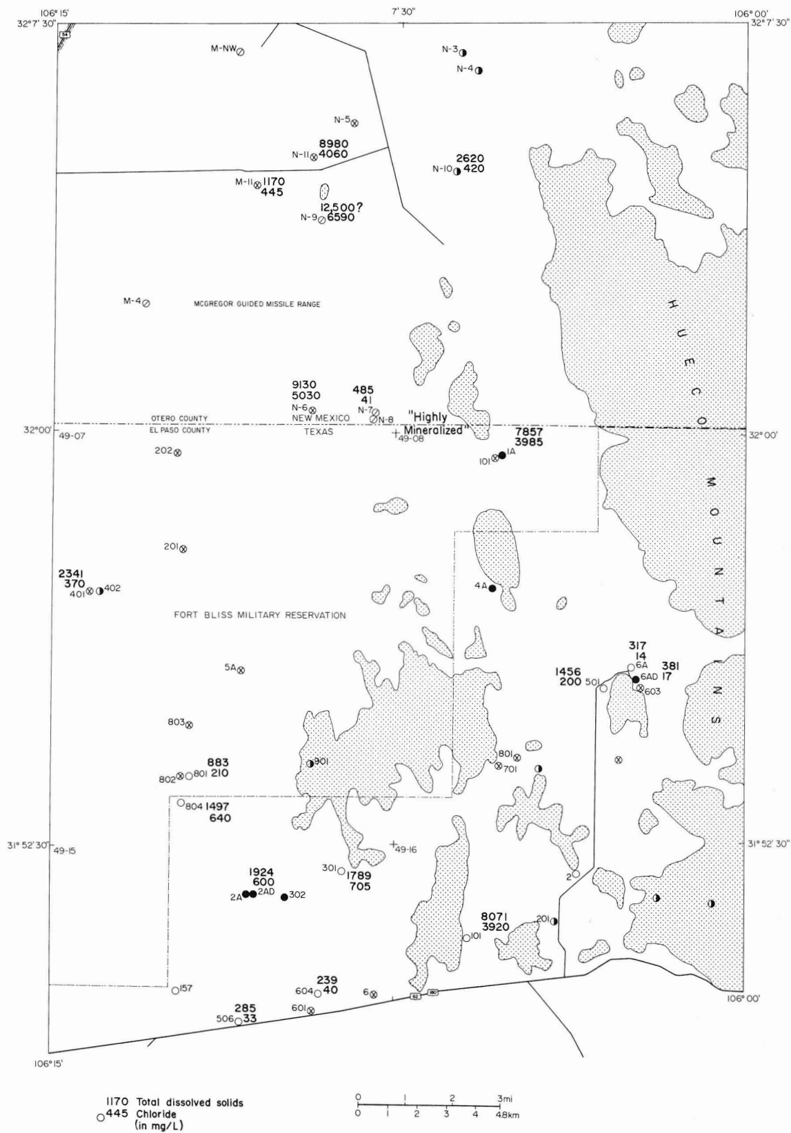
Figure 9. Total dissolved solids and chloride concentrations.
