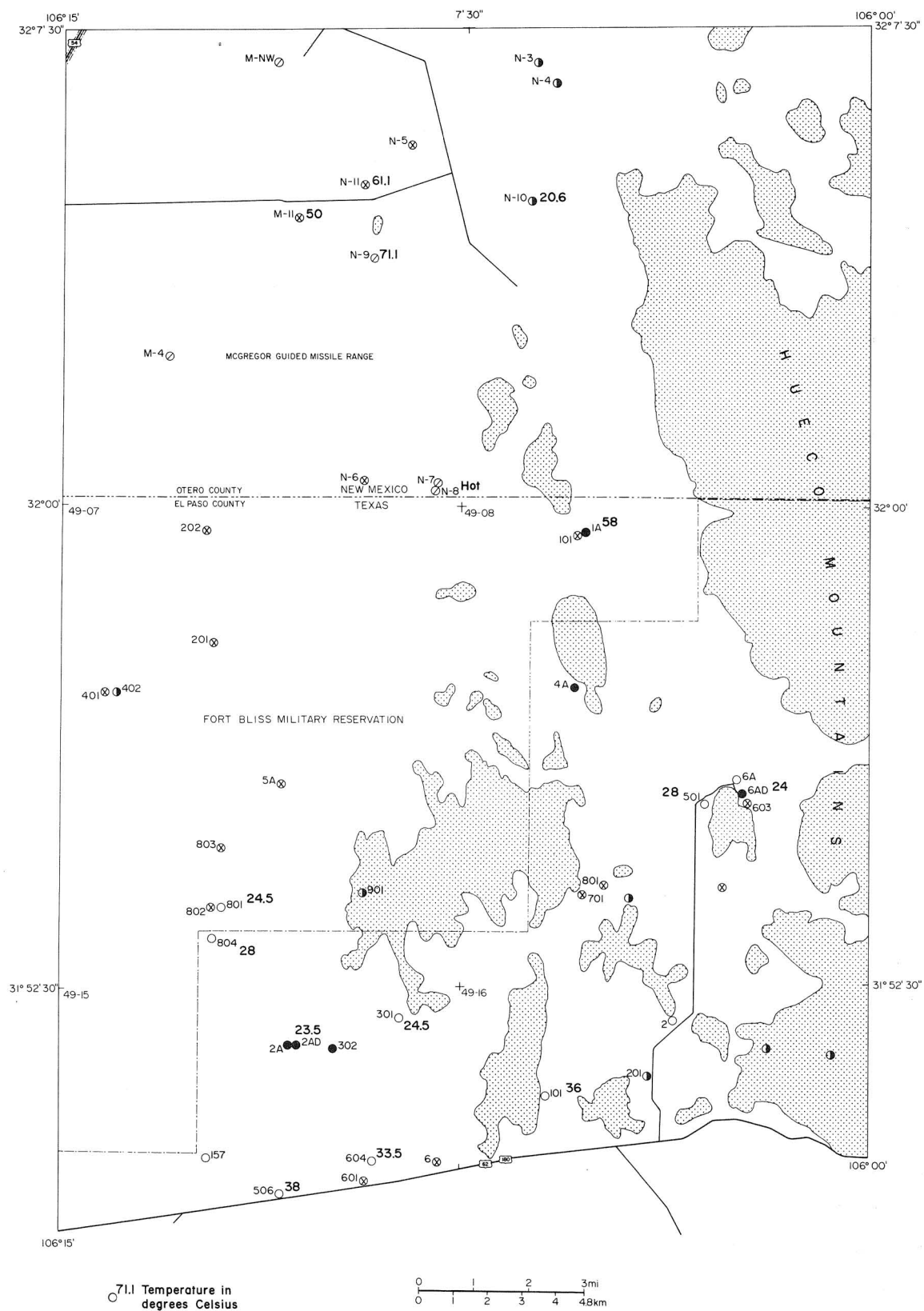
Figure 3. Measured and reported temperatures (°C) of thermal and nonthermal wells.
