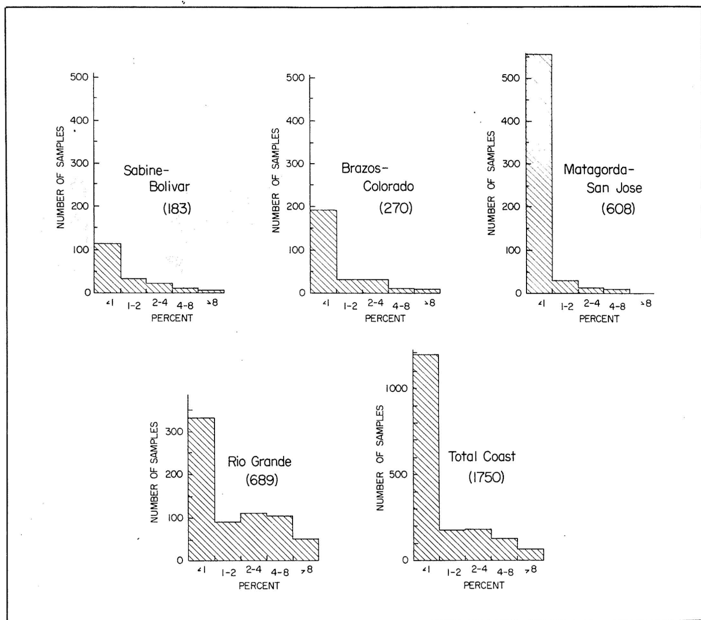
Figure 6. Frequency distribution of percent coarse fraction in each of the four trends and for all samples studied. Total number of samples shown in parentheses.
