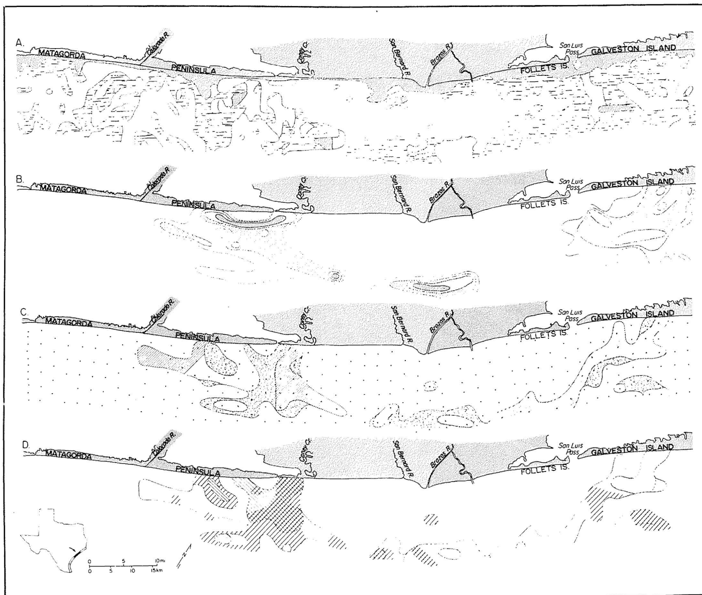
Figure 2. Maps of the Brazos-Colorado area showing: A) surface sediment distribution; B) coarse fraction percent by volume; C) rock fragments; and D) restricted mollusc species. Symbols explained on figure 1.
