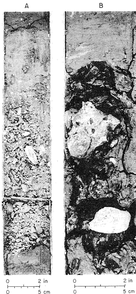
Figure 7. Cores from the Matagorda-San Jose trend showing: 1) shelf deposits overlying estuarine sediments with abundant oyster shells; and 2) graded bedding interpreted as a storm deposit.
