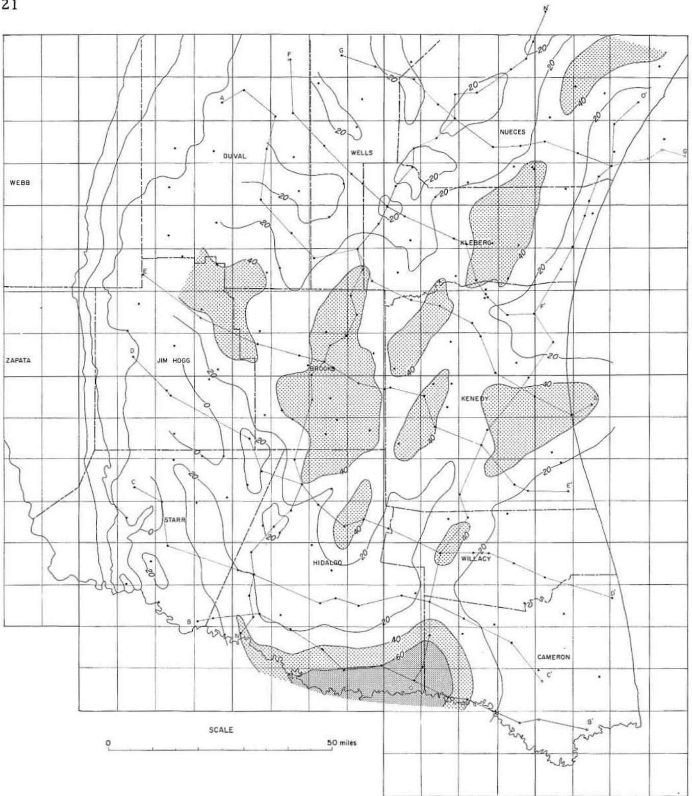
Fig. 15. Sand percentage in zone T4-T5.
