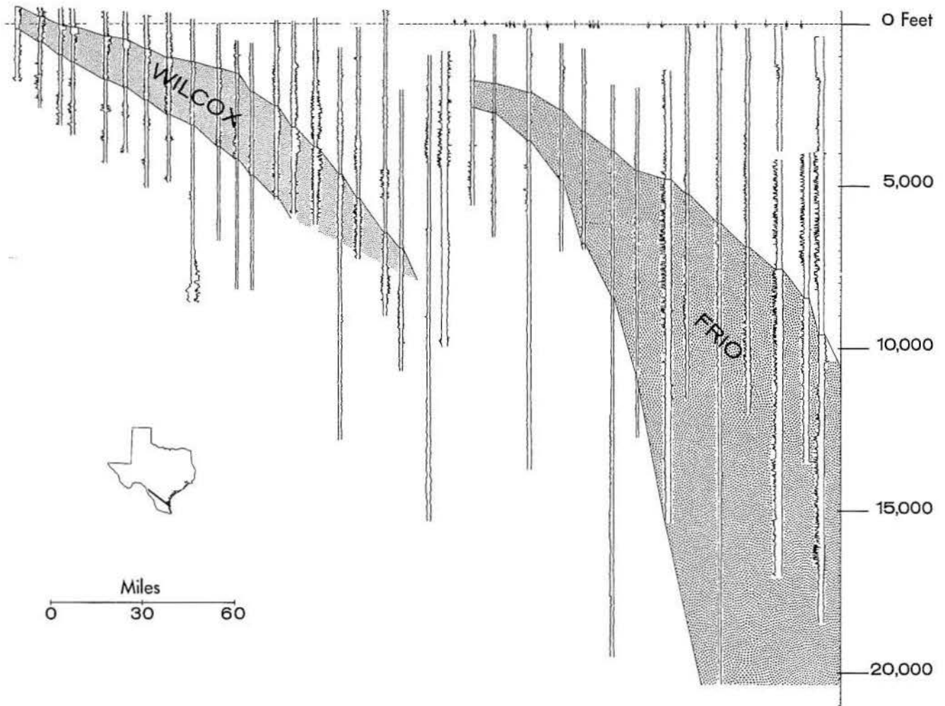
Fig. 4. Regional cross section on a sea-level datum showing the pattern of sand-shale packages offlapping toward the coast.
