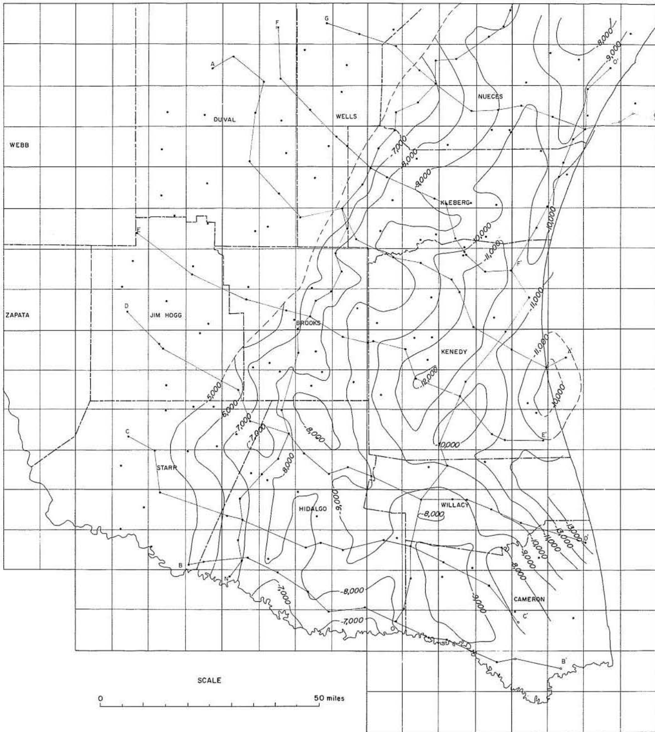
Fig. 21. Top of the geopressed zone, South Texas.
