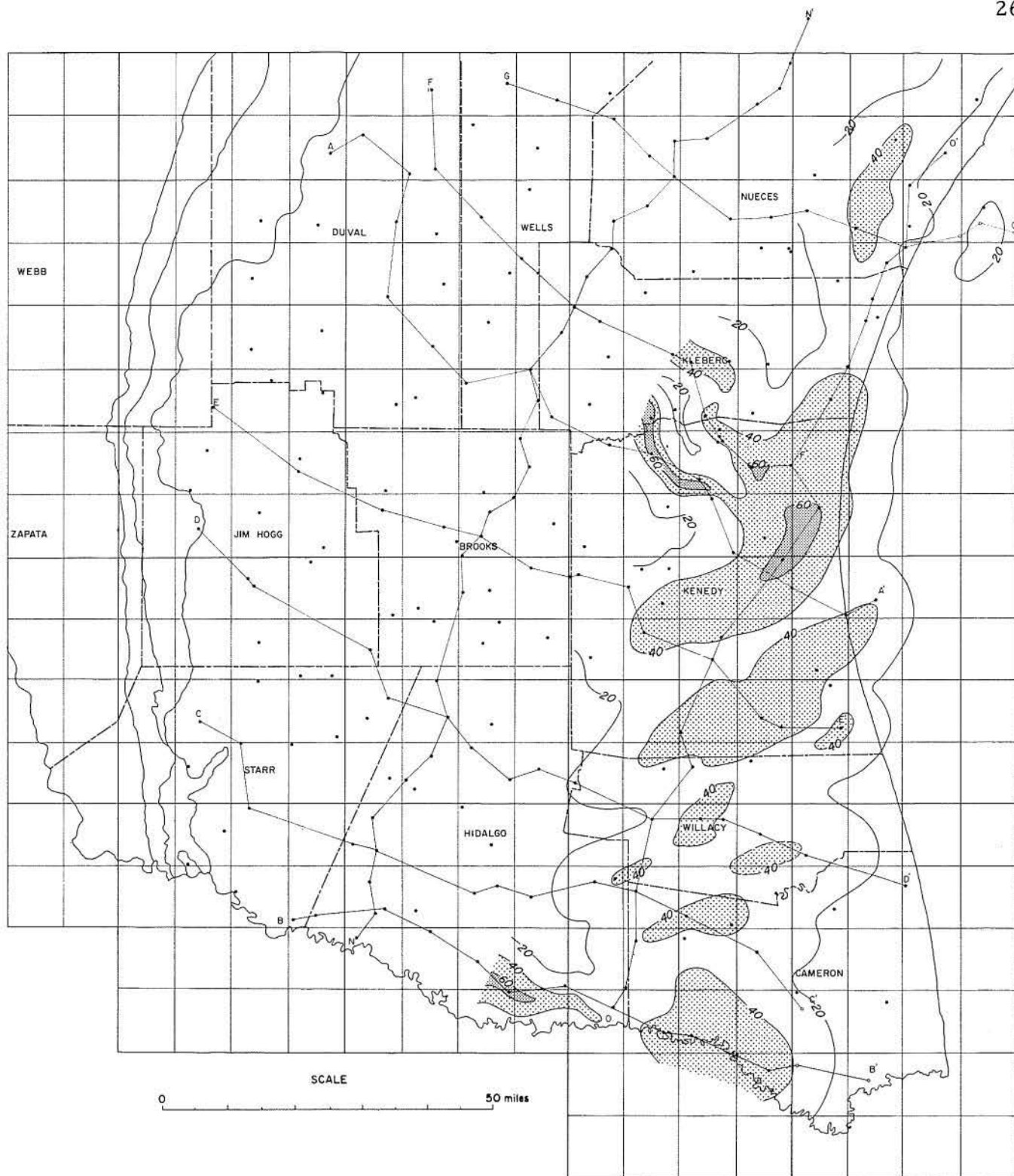
Fig. 20. Sand percentage in zone T0-T1.
