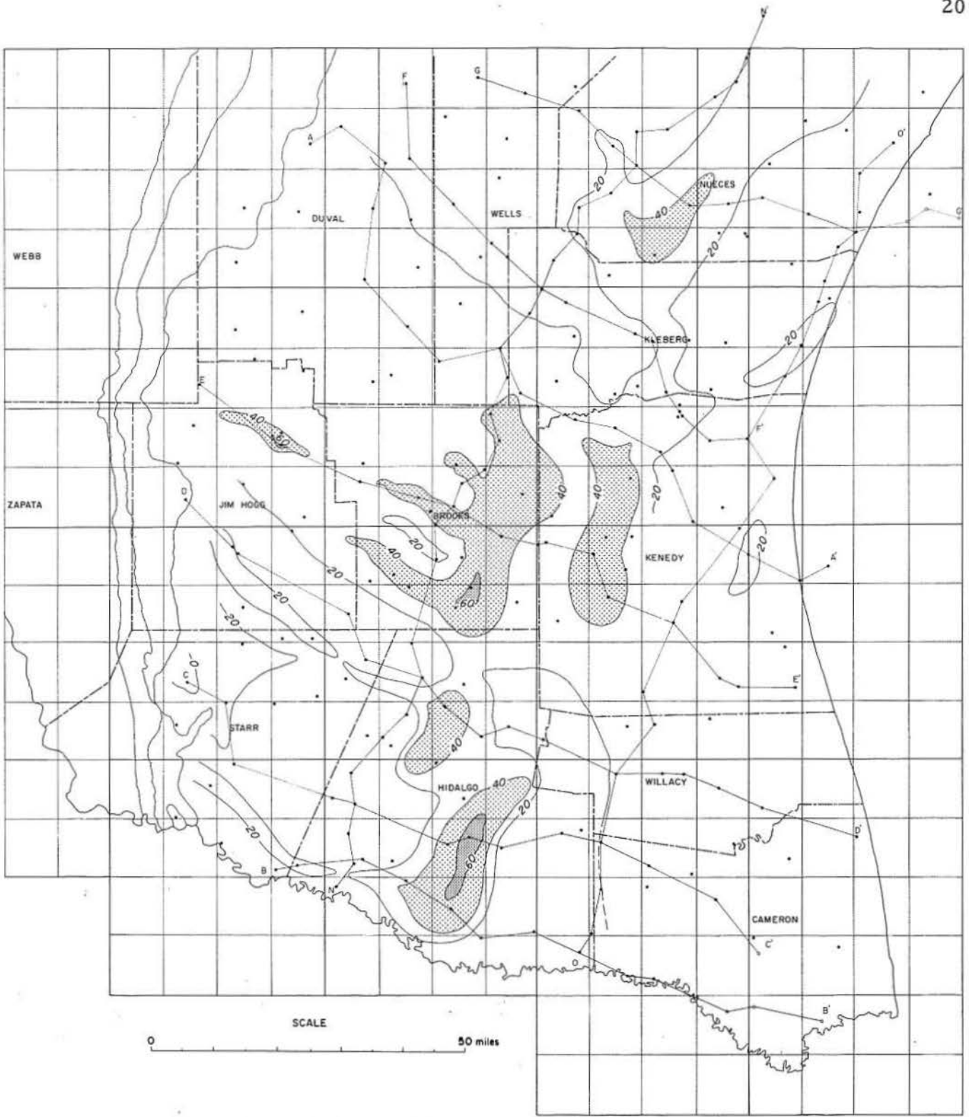
Fig. 14. Sand percentage in zone T5-T6.
