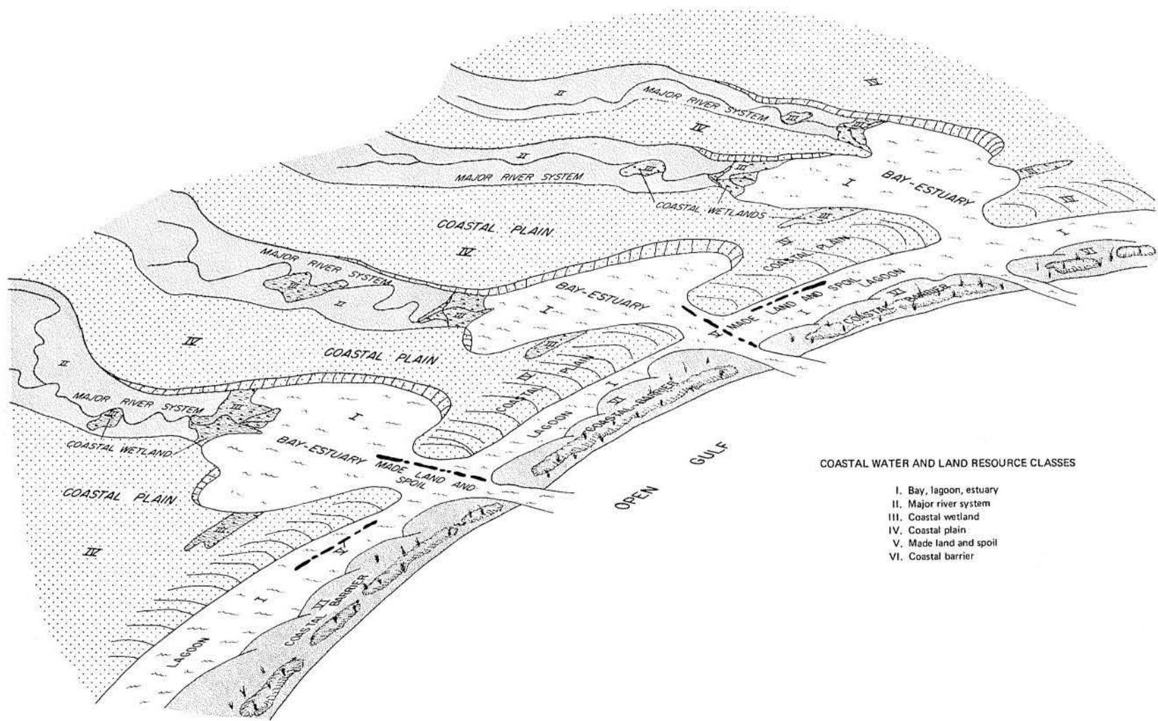
FIG. 1. Schematic map of major land and water resource capability classes, Texas Coastal Zone.
