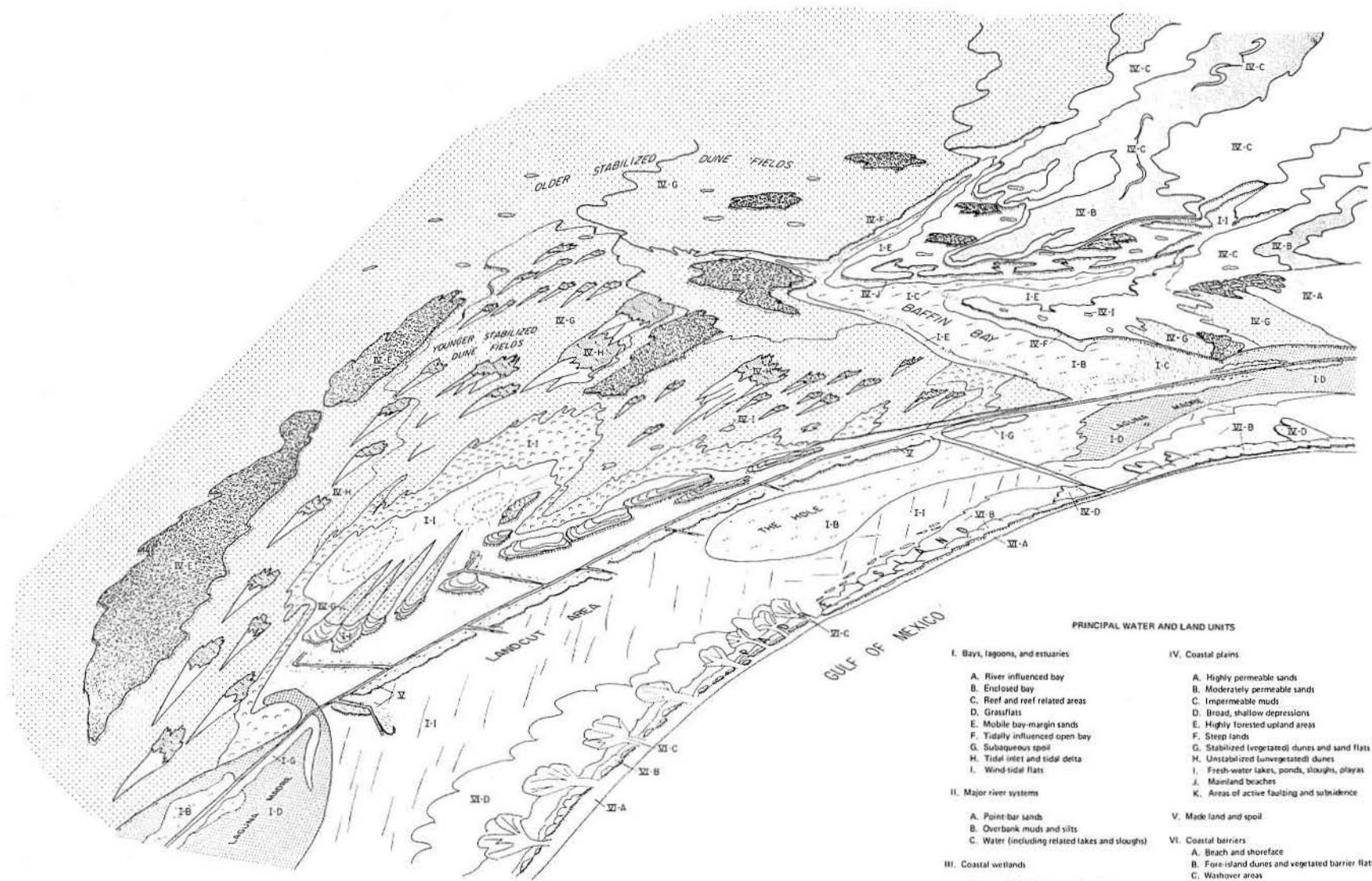
FIG. 4. Schematic map of land and water resource capability units, arid south Texas Coastal Zone.
