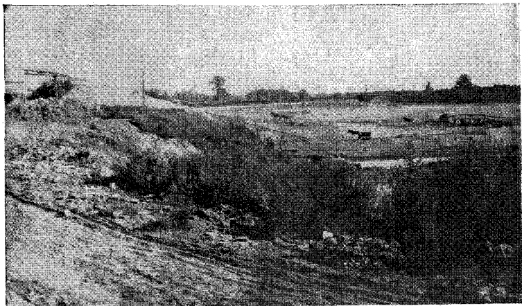
FIG. 4. CLAY EXCAVATION BY HORSE-DRAWN SHOVEL SCRAPERS IN THE PIT OF A DALLAS, TEXAS, BRICK PLANT
