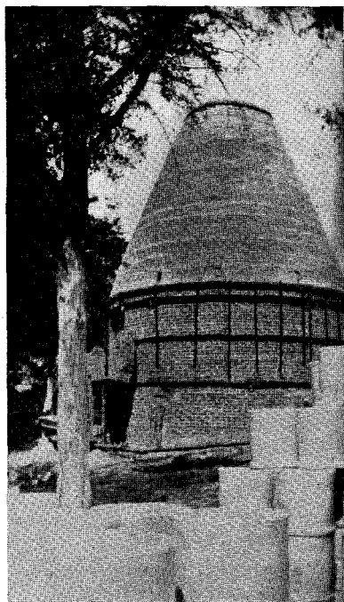
FIG. 9. UPDRAFT MUFFLE TYPE OF BEEHIVE KILN USED IN BURNING POTTERY
