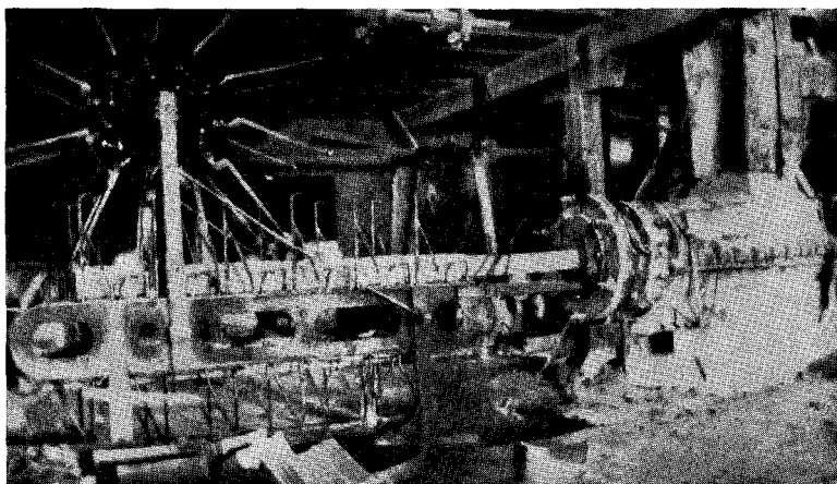
FIG. 8. STEP IN THE FORMING OF HOLLOW TILE. CLAY COLUMN COMING FROM THE AUGER MACHINE ON TO THE CUTTING TABLE AT AN ATHENS, TEXAS, PLANT
