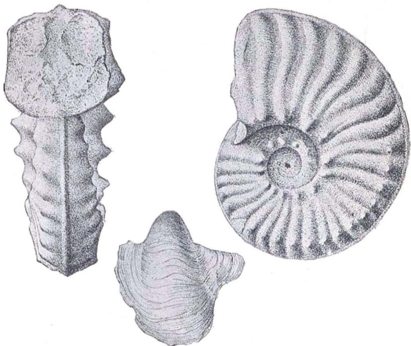
Plate I. Left side: Ammonites Conensis Roemer. From the Fort Worth Limestone. Right side: Same; a side view. Below: Gryphaea Washitaensis Hill. From the Dennison beds.
