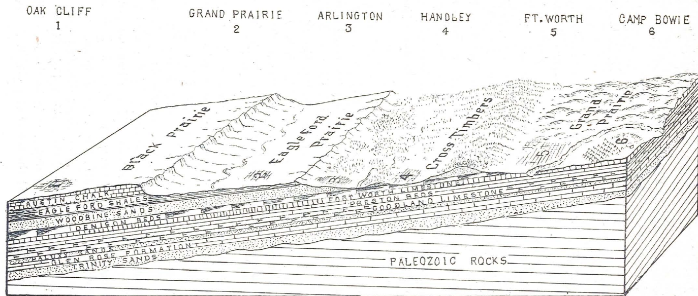
Figure 1. Block diagram showing the underground structure and surface topography, the cuestas, in the vicinity of Camp Bowie.
