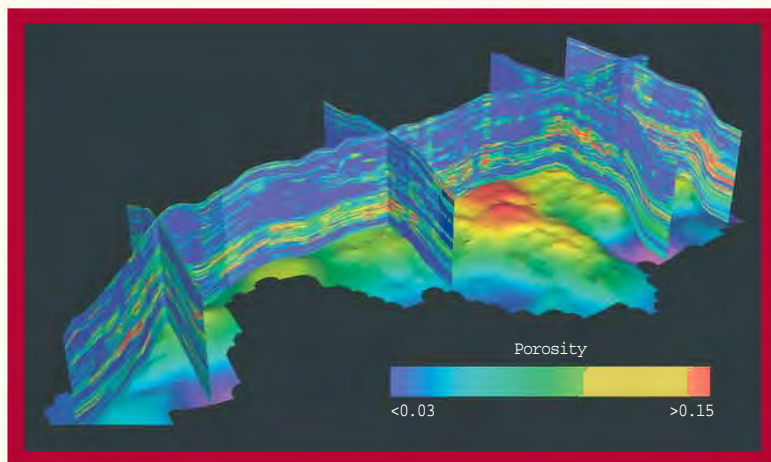
Porosity distribution in Fullerton Clear Fork Unit, Andrews County, West Texas. The model, created using reservoir modeling software, lies atop the structure base map.
