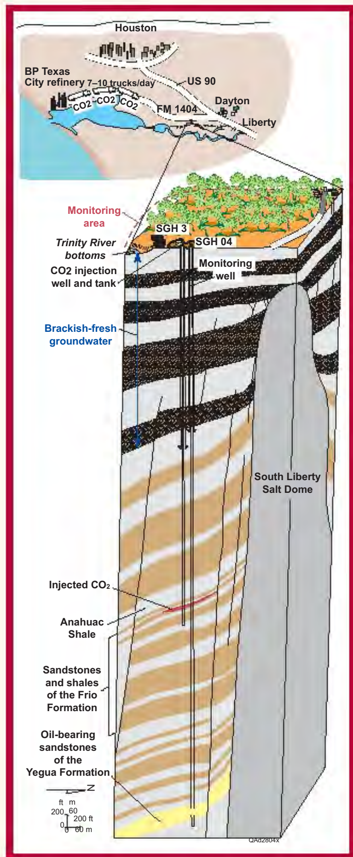
True-scale diagram of CO 2 injection into a brine-bearing sandstone of the upper Frio Formation.
