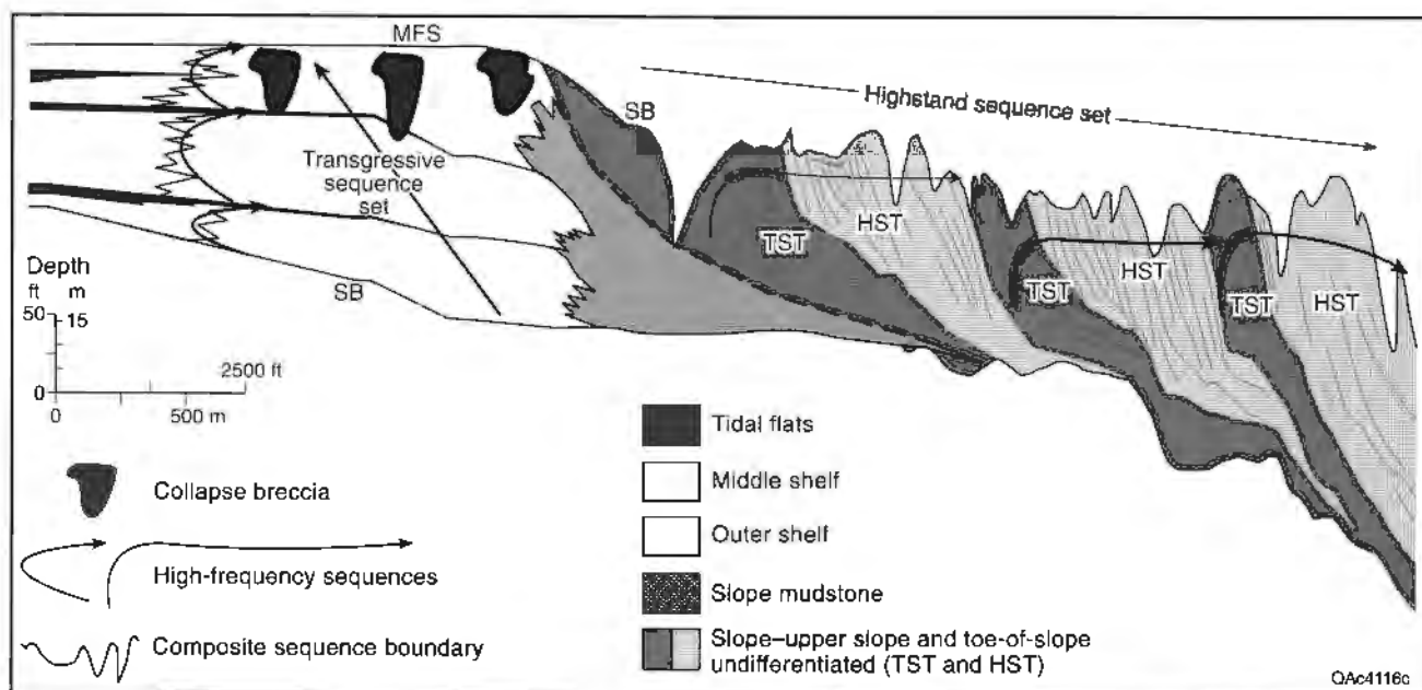
Outcrop-analog model of coastal paleokarst, Lower Permian, Apache Canyon, Sierra Diablo Range, West Texas. Knowledge of distribution of karst features relative to high-resolution sequence framework helps researchers in subsurface prediction of paleokarst development. SB=composite sequence boundary, MFS=maximum flooding surface, TST=transgressive systems tract, HST=highstand systems tract.
