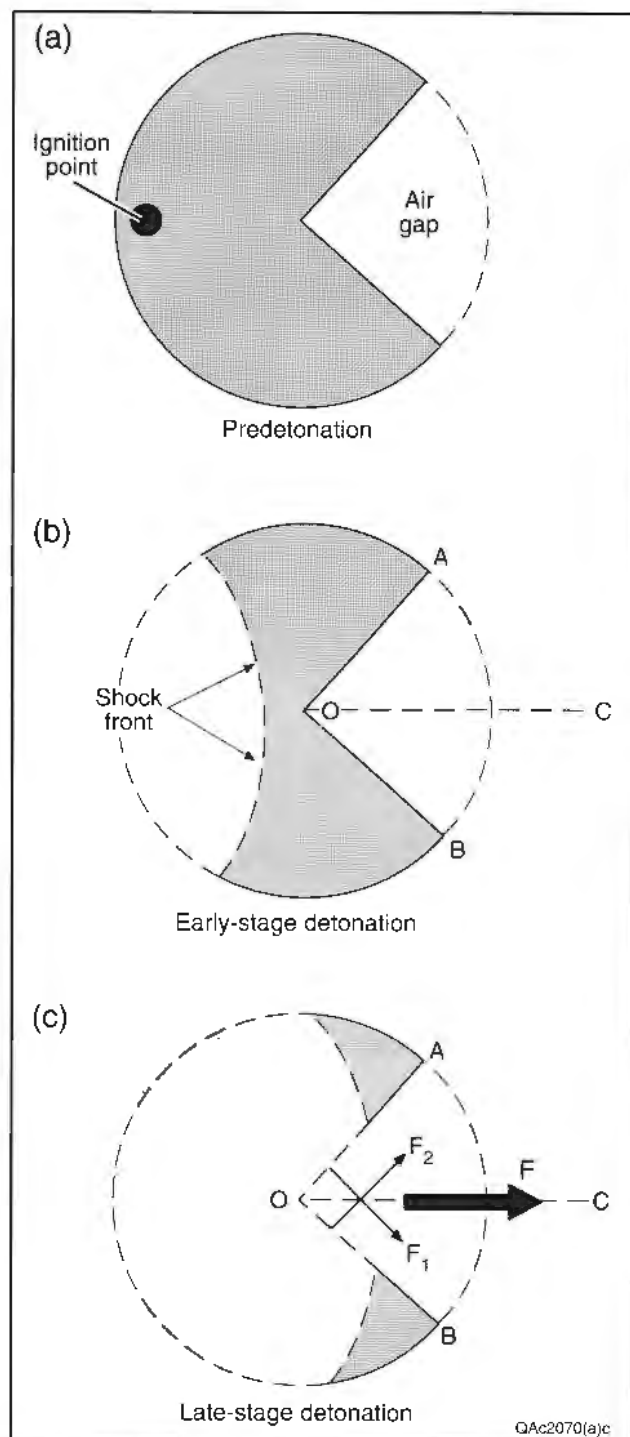
Diagram showing stages of detonation of directional, shaped-charge, seismic explosive package developed by Bureau researchers for the Henderson Dome study. This package allows operators to generate seismic S-waves (essential for detection of fractured reservoir facies) in prospect areas where conventional S-wave sources cannot be used. The overhead view in the diagram allows us to look down on the shaped charge as it proceeds through three stages of detonation. The detonation front is created at (a) an ignition point that is directly opposite (b) the shaped notch BOA. As the shock front sweeps past (c) the notch, it creates counteropposed forces F_1 and F_2 that sum as vectors to create a strong horizontal force, F . The shaped notch extends the full length of the cylindrical charge.
