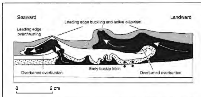
Cross section of a physical model showing complex deformation at the leading edge of originally extrusive salt sheets (black). Deformation is driven by gravitational loading by a prograding sedimentary wedge off section to the right. Similar structures are widespread in former slope environments in the Gulf of Mexico.
