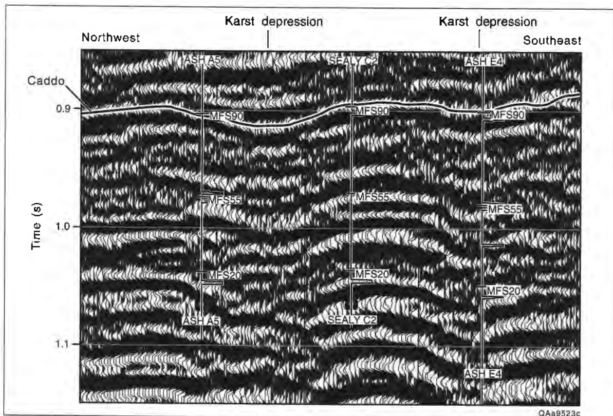
Seismic profile of Boonsville field in the Fort Worth Basin, part of a 3-D seismic data volume, showing the genetic relation between the compartmentalization of siliciclastic reservoirs and karst depressions created by dissolution of deeper carbonates. The Caddo horizon is the top of the productive Bend Conglomerate section and is more than 2,000 ft above the Ellenburger carbonates, where the karsting occurred. Production data show that the structural high between the two karst depressions contains a Caddo sandstone reservoir.
